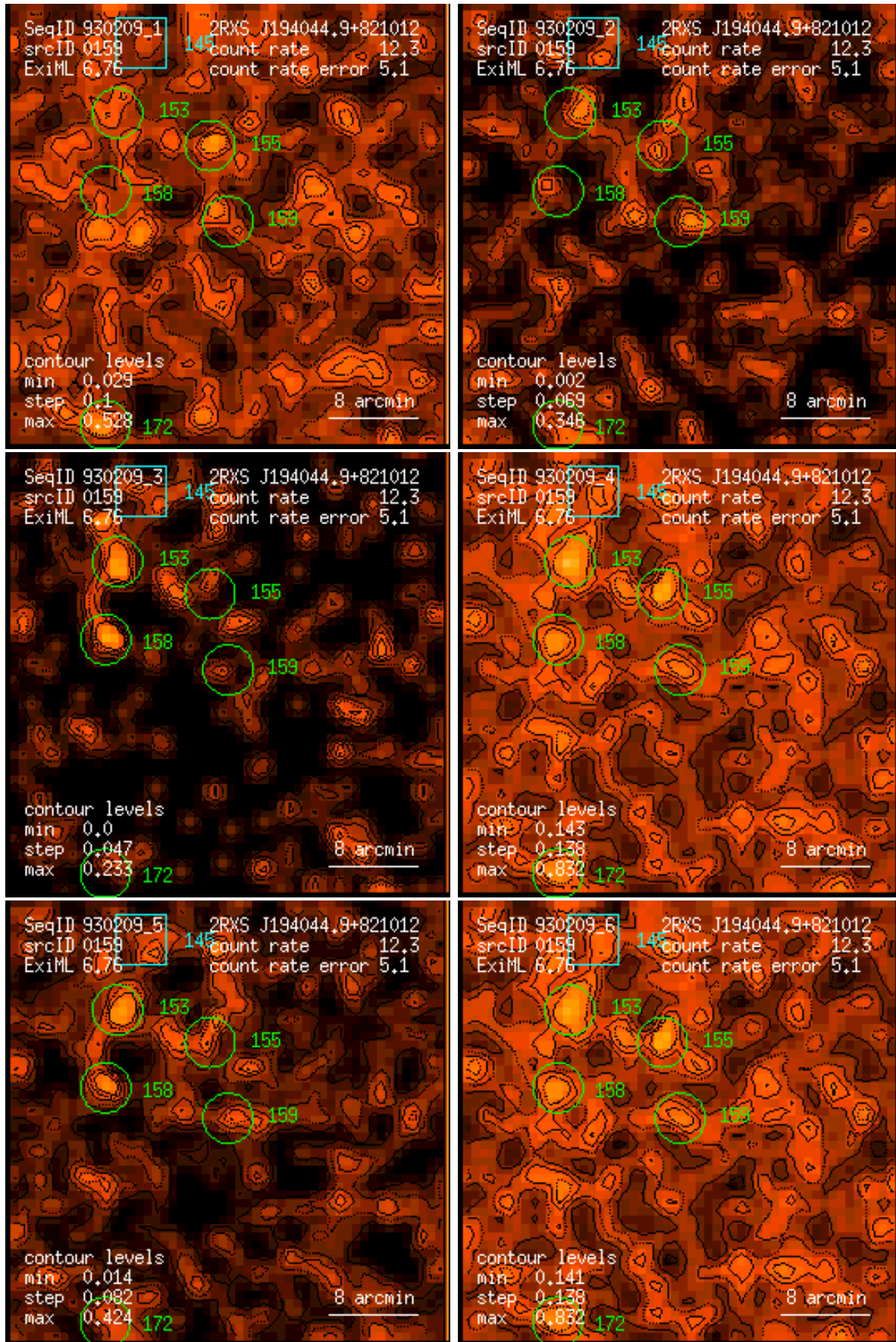
Figure 159: RASS 930209: detection 0159: band rate images, Gaussian filter: (1) PSPC channels 11 – 41, (2) 52 – 90, (3) 91 – 201, (4) 11 – 235, (5) 52 – 201, (6) 11 – 201. Broad band rates in counts/ks. Band rate contour levels in counts/ks/arcmin 2 .
