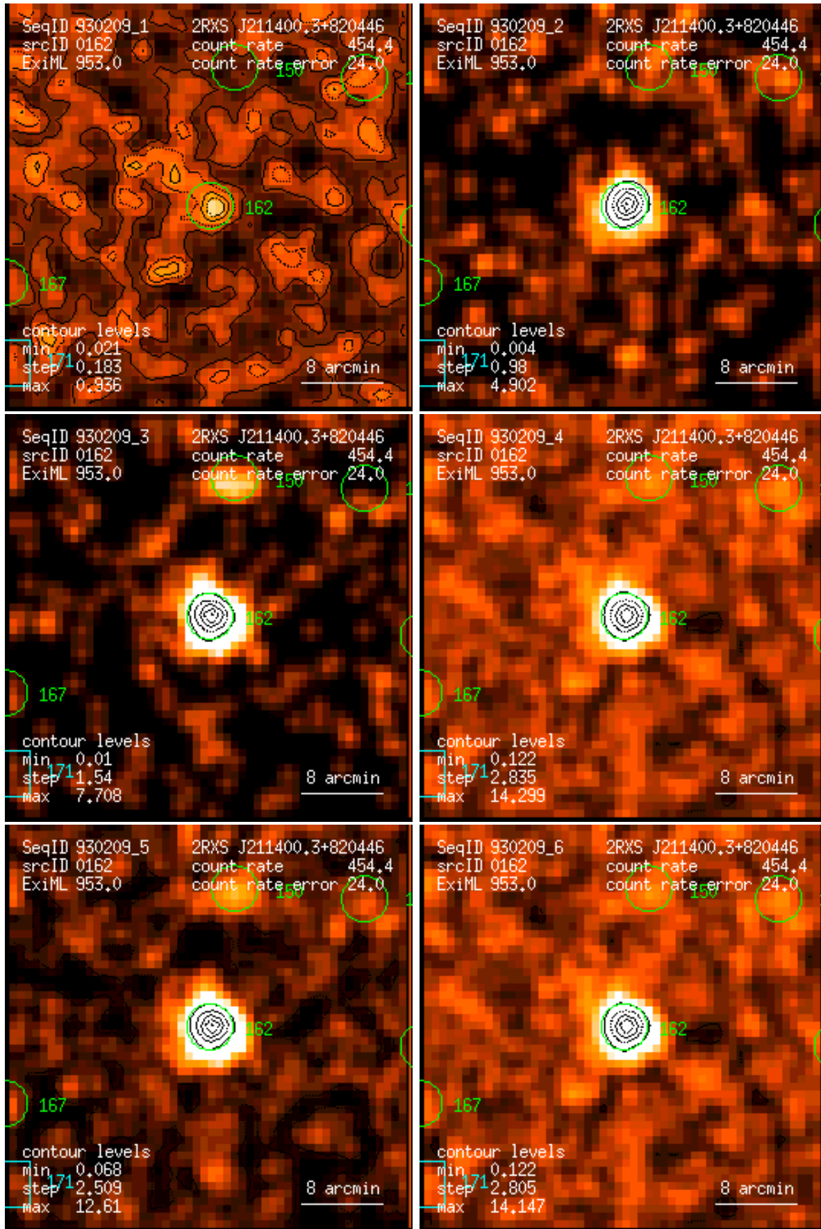
Figure 162: RASS 930209: detection 0162: band rate images, Gaussian filter: (1) PSPC channels 11 – 41, (2) 52 – 90, (3) 91 – 201, (4) 11 – 235, (5) 52 – 201, (6) 11 – 201. Broad band rates in counts/ks. Band rate contour levels in counts/ks/arcmin 2 .
