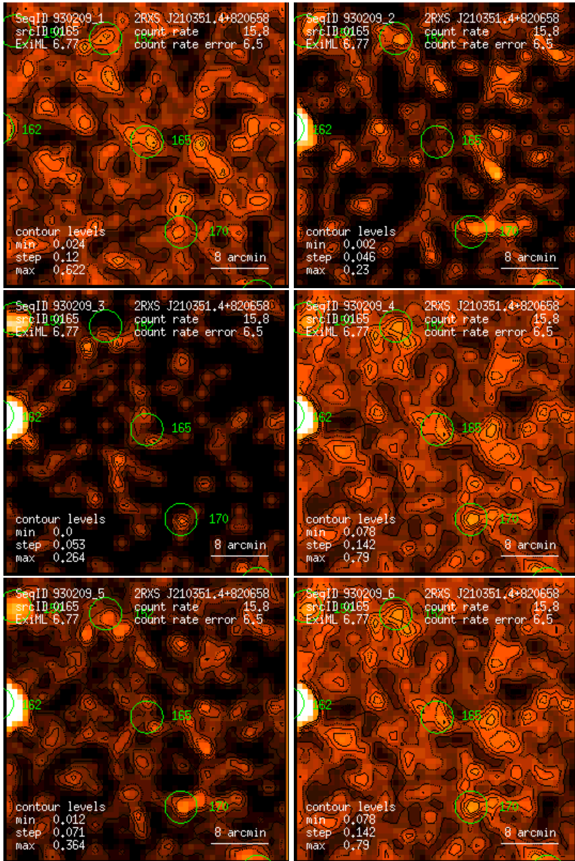
Figure 165: RASS 930209: detection 0165: band rate images, Gaussian filter: (1) PSPC channels 11 – 41, (2) 52 – 90, (3) 91 – 201, (4) 11 – 235, (5) 52 – 201, (6) 11 – 201. Broad band rates in counts/ks. Band rate contour levels in counts/ks/arcmin 2 .
