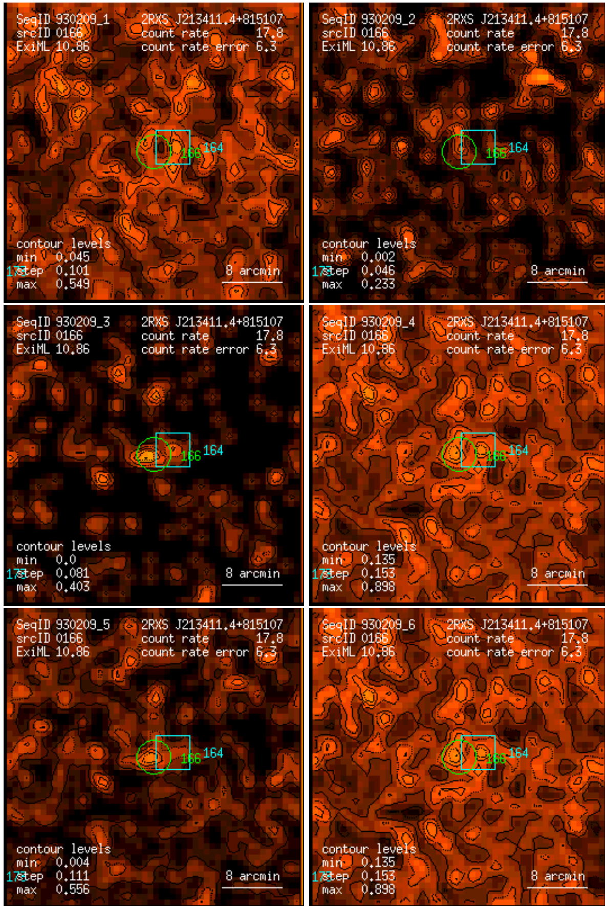
Figure 166: RASS 930209: detection 0166: band rate images, Gaussian filter: (1) PSPC channels 11 – 41, (2) 52 – 90, (3) 91 – 201, (4) 11 – 235, (5) 52 – 201, (6) 11 – 201. Broad band rates in counts/ks. Band rate contour levels in counts/ks/arcmin 2 .
