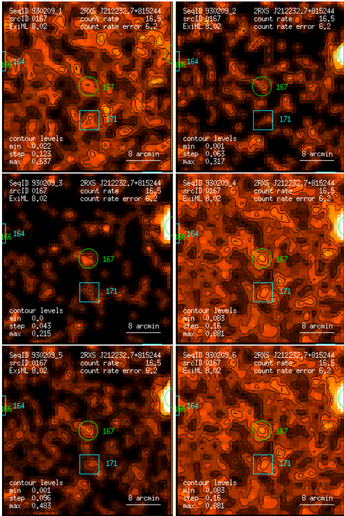
Figure 167: RASS 930209: detection 0167: band rate images, Gaussian filter: (1) PSPC channels 11 – 41, (2) 52 – 90, (3) 91 – 201, (4) 11 – 235, (5) 52 – 201, (6) 11 – 201. Broad band rates in counts/ks. Band rate contour levels in counts/ks/arcmin 2 .
