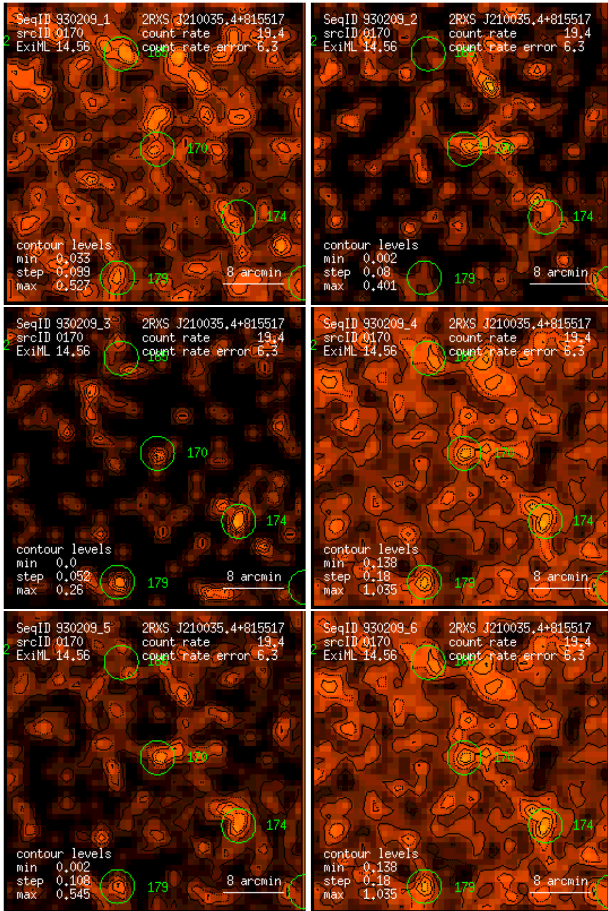
Figure 170: RASS 930209: detection 0170: band rate images, Gaussian filter: (1) PSPC channels 11 – 41, (2) 52 – 90, (3) 91 – 201, (4) 11 – 235, (5) 52 – 201, (6) 11 – 201. Broad band rates in counts/ks. Band rate contour levels in counts/ks/arcmin 2 .
