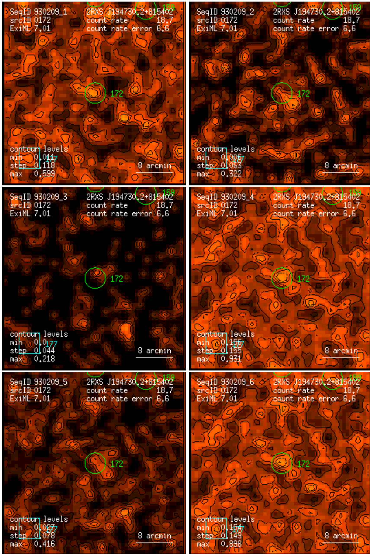
Figure 172: RASS 930209: detection 0172: band rate images, Gaussian filter: (1) PSPC channels 11 – 41, (2) 52 – 90, (3) 91 – 201, (4) 11 – 235, (5) 52 – 201, (6) 11 – 201. Broad band rates in counts/ks. Band rate contour levels in counts/ks/arcmin 2 .
