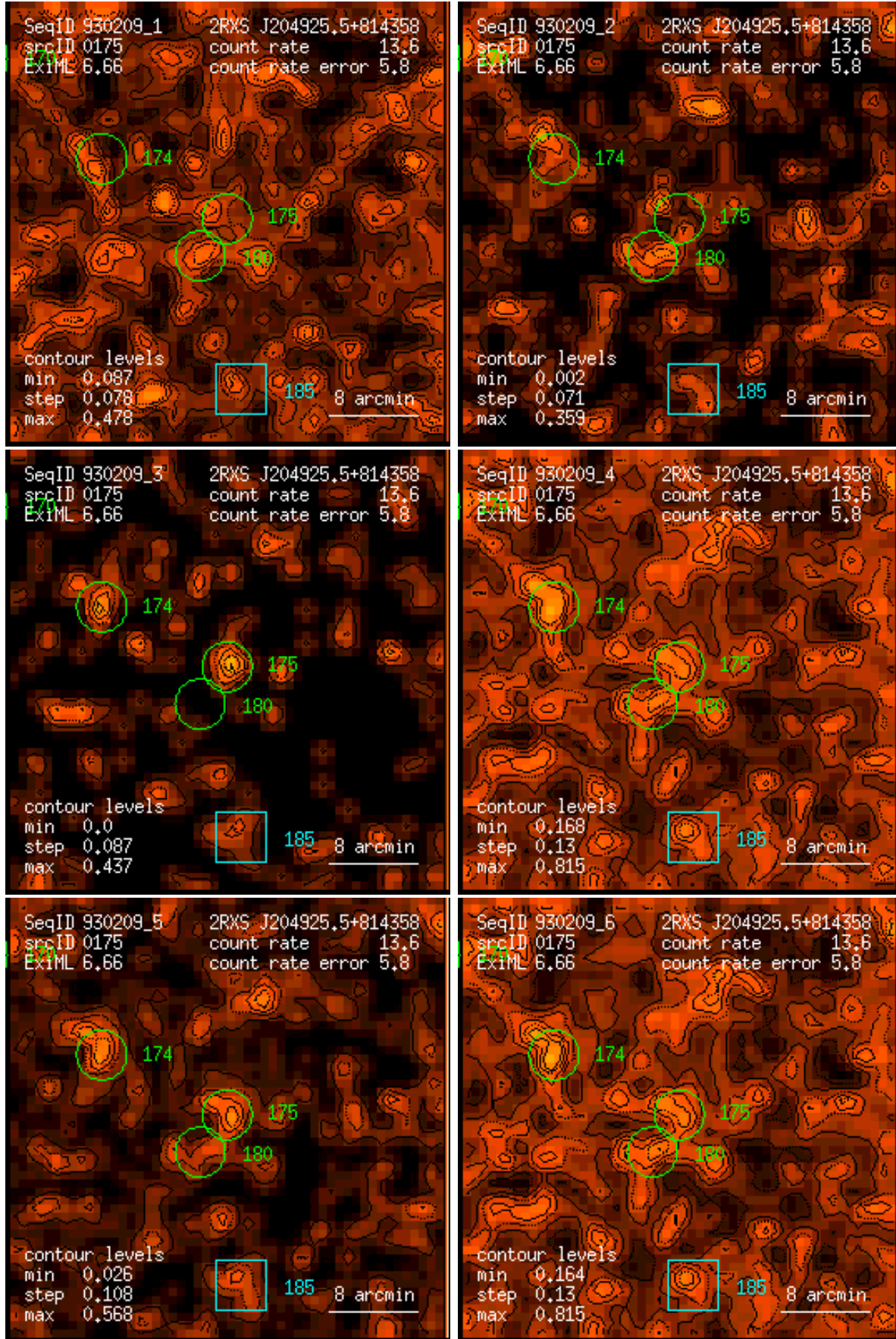
Figure 175: RASS 930209: detection 0175: band rate images, Gaussian filter: (1) PSPC channels 11 – 41, (2) 52 – 90, (3) 91 – 201, (4) 11 – 235, (5) 52 – 201, (6) 11 – 201. Broad band rates in counts/ks. Band rate contour levels in counts/ks/arcmin 2 .
