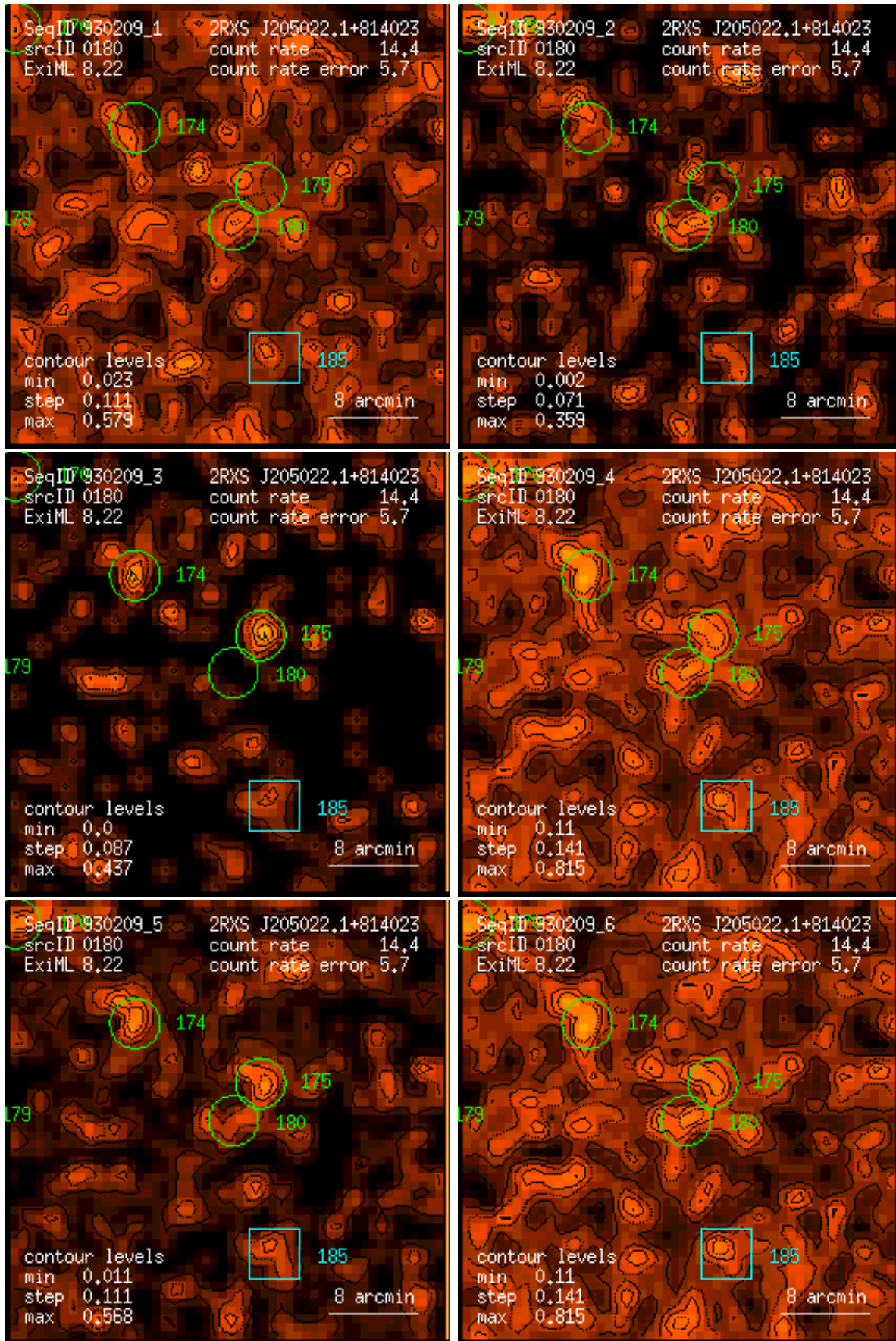
Figure 180: RASS 930209: detection 0180: band rate images, Gaussian filter: (1) PSPC channels 11 – 41, (2) 52 – 90, (3) 91 – 201, (4) 11 – 235, (5) 52 – 201, (6) 11 – 201. Broad band rates in counts/ks. Band rate contour levels in counts/ks/arcmin 2 .
