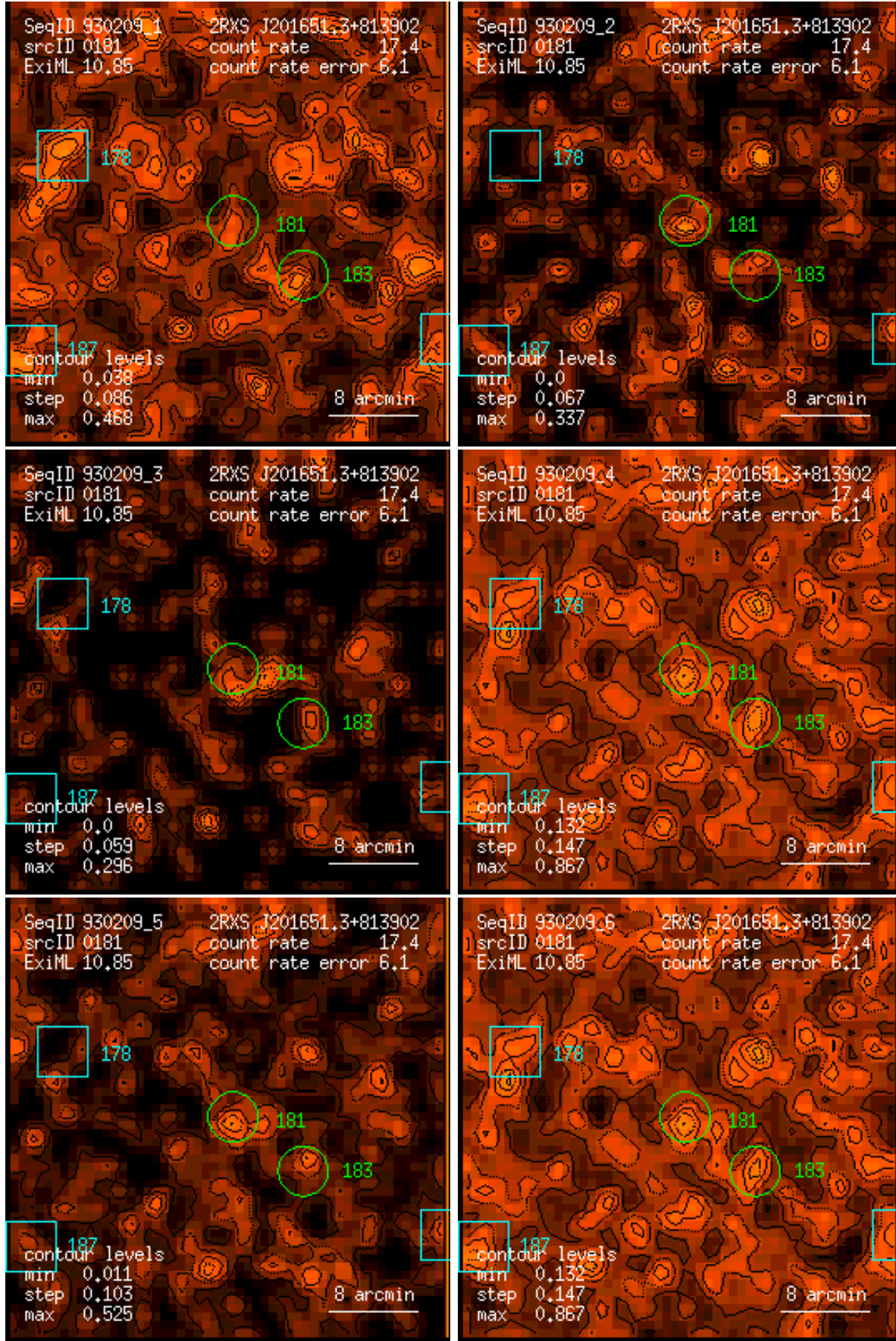
Figure 181: RASS 930209: detection 0181: band rate images, Gaussian filter: (1) PSPC channels 11 – 41, (2) 52 – 90, (3) 91 – 201, (4) 11 – 235, (5) 52 – 201, (6) 11 – 201. Broad band rates in counts/ks. Band rate contour levels in counts/ks/arcmin 2 .
