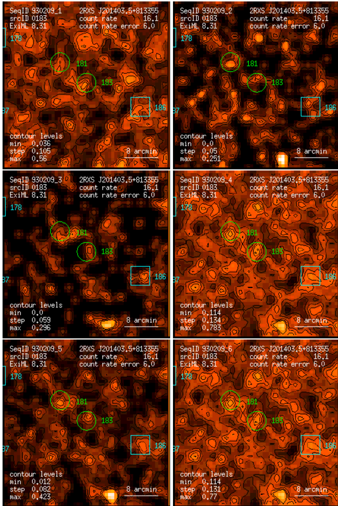
Figure 183: RASS 930209: detection 0183: band rate images, Gaussian filter: (1) PSPC channels 11 – 41, (2) 52 – 90, (3) 91 – 201, (4) 11 – 235, (5) 52 – 201, (6) 11 – 201. Broad band rates in counts/ks. Band rate contour levels in counts/ks/arcmin 2 .
