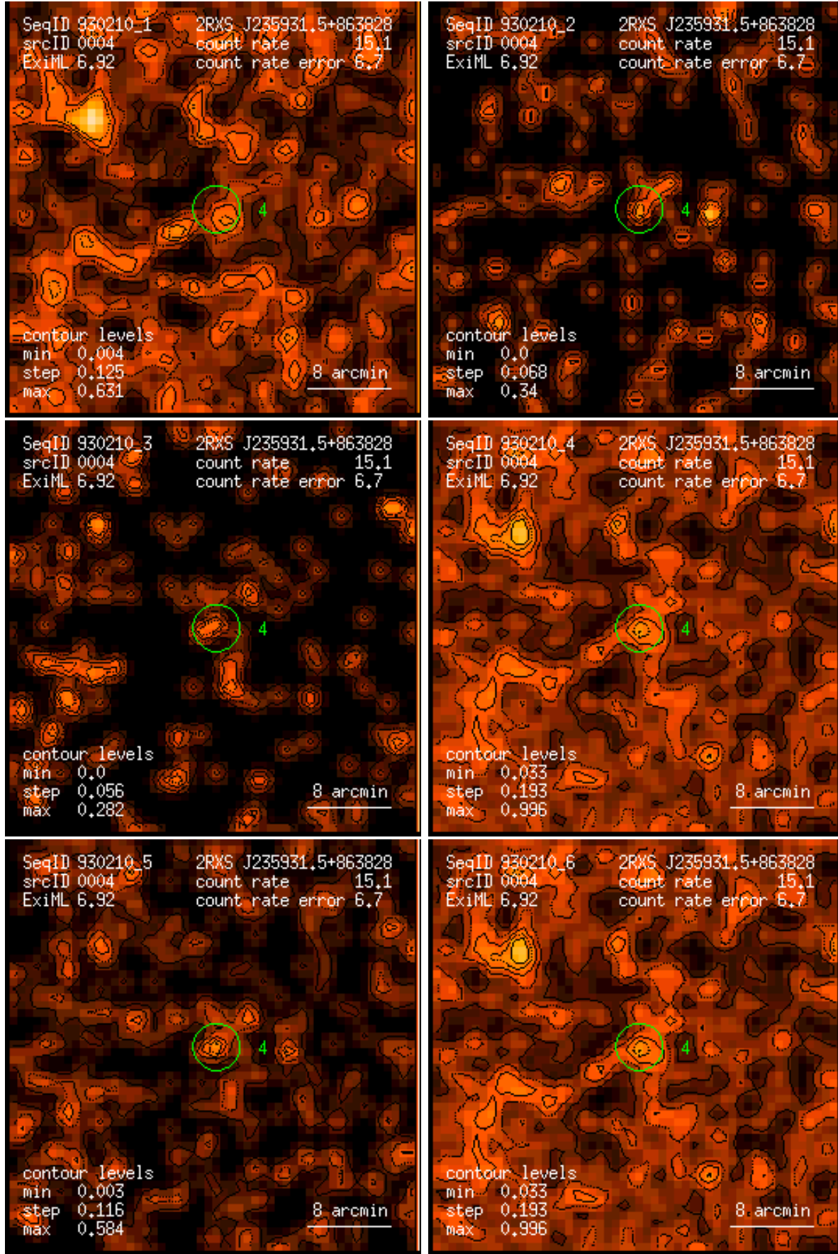
Figure 4: RASS 930210: detection 0004: band rate images, Gaussian filter: (1) PSPC channels 11 – 41, (2) 52 – 90, (3) 91 – 201, (4) 11 – 235, (5) 52 – 201, (6) 11 – 201. Broad band rates in counts/ks. Band rate contour levels in counts/ks/arcmin 2 .
