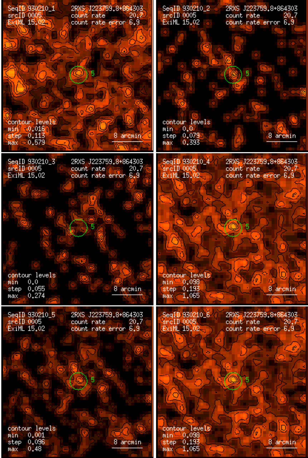
Figure 5: RASS 930210: detection 0005: band rate images, Gaussian filter: (1) PSPC channels 11 – 41, (2) 52 – 90, (3) 91 – 201, (4) 11 – 235, (5) 52 – 201, (6) 11 – 201. Broad band rates in counts/ks. Band rate contour levels in counts/ks/arcmin 2 .
