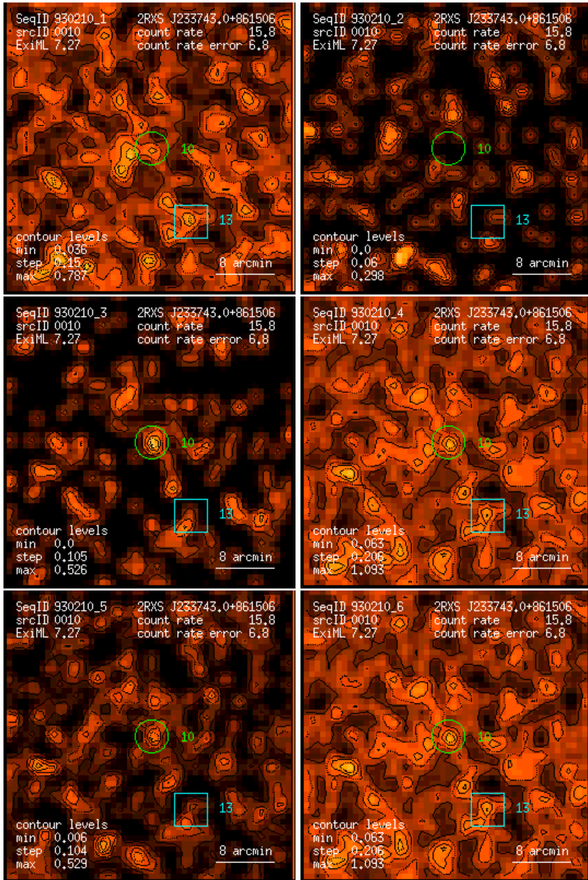
Figure 10: RASS 930210: detection 0010: band rate images, Gaussian filter: (1) PSPC channels 11 – 41, (2) 52 – 90, (3) 91 – 201, (4) 11 – 235, (5) 52 – 201, (6) 11 – 201. Broad band rates in counts/ks. Band rate contour levels in counts/ks/arcmin 2 .
