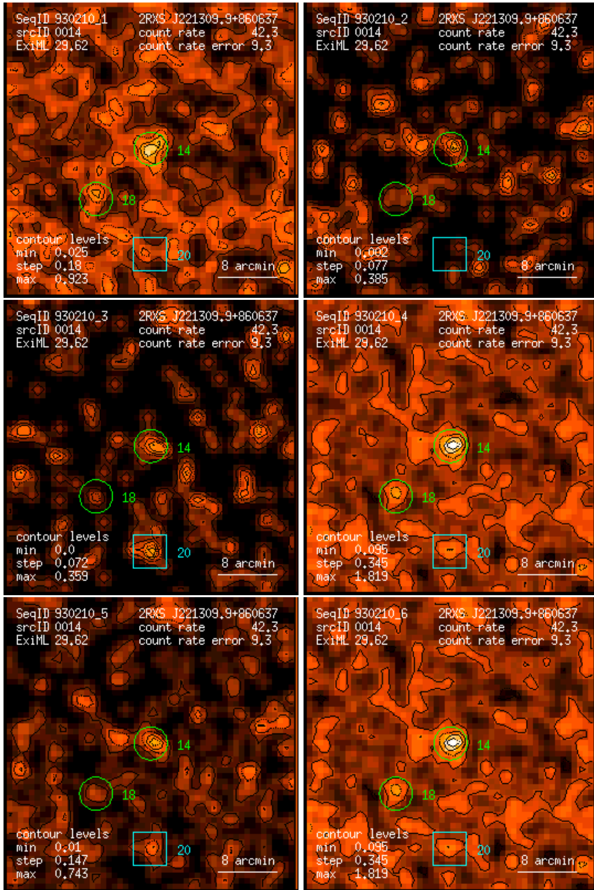
Figure 14: RASS 930210: detection 0014: band rate images, Gaussian filter: (1) PSPC channels 11 – 41, (2) 52 – 90, (3) 91 – 201, (4) 11 – 235, (5) 52 – 201, (6) 11 – 201. Broad band rates in counts/ks. Band rate contour levels in counts/ks/arcmin 2 .
