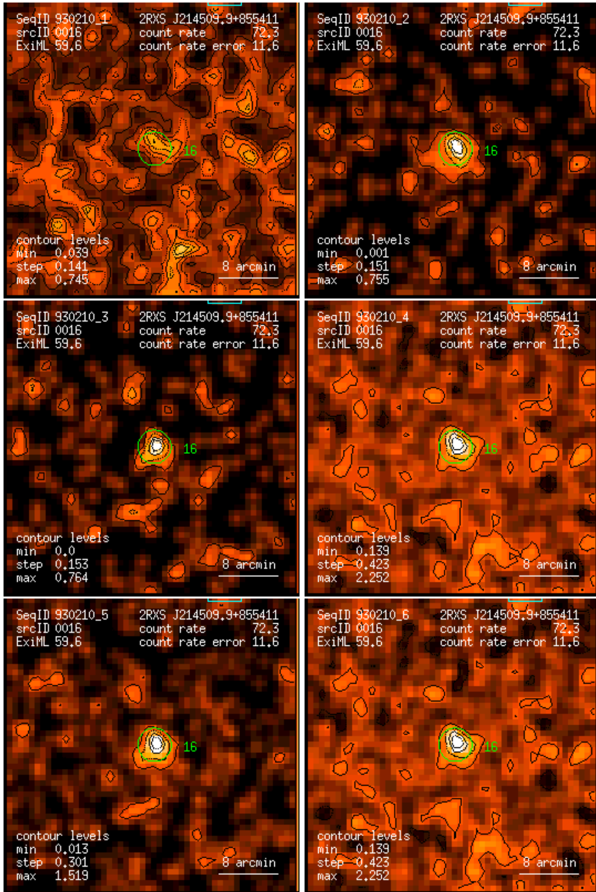
Figure 16: RASS 930210: detection 0016: band rate images, Gaussian filter: (1) PSPC channels 11 – 41, (2) 52 – 90, (3) 91 – 201, (4) 11 – 235, (5) 52 – 201, (6) 11 – 201. Broad band rates in counts/ks. Band rate contour levels in counts/ks/arcmin 2 .
