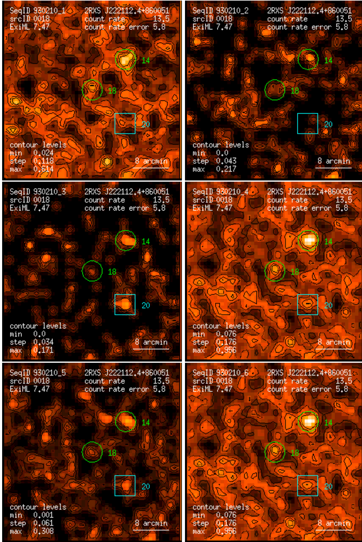
Figure 18: RASS 930210: detection 0018: band rate images, Gaussian filter: (1) PSPC channels 11 – 41, (2) 52 – 90, (3) 91 – 201, (4) 11 – 235, (5) 52 – 201, (6) 11 – 201. Broad band rates in counts/ks. Band rate contour levels in counts/ks/arcmin 2 .
