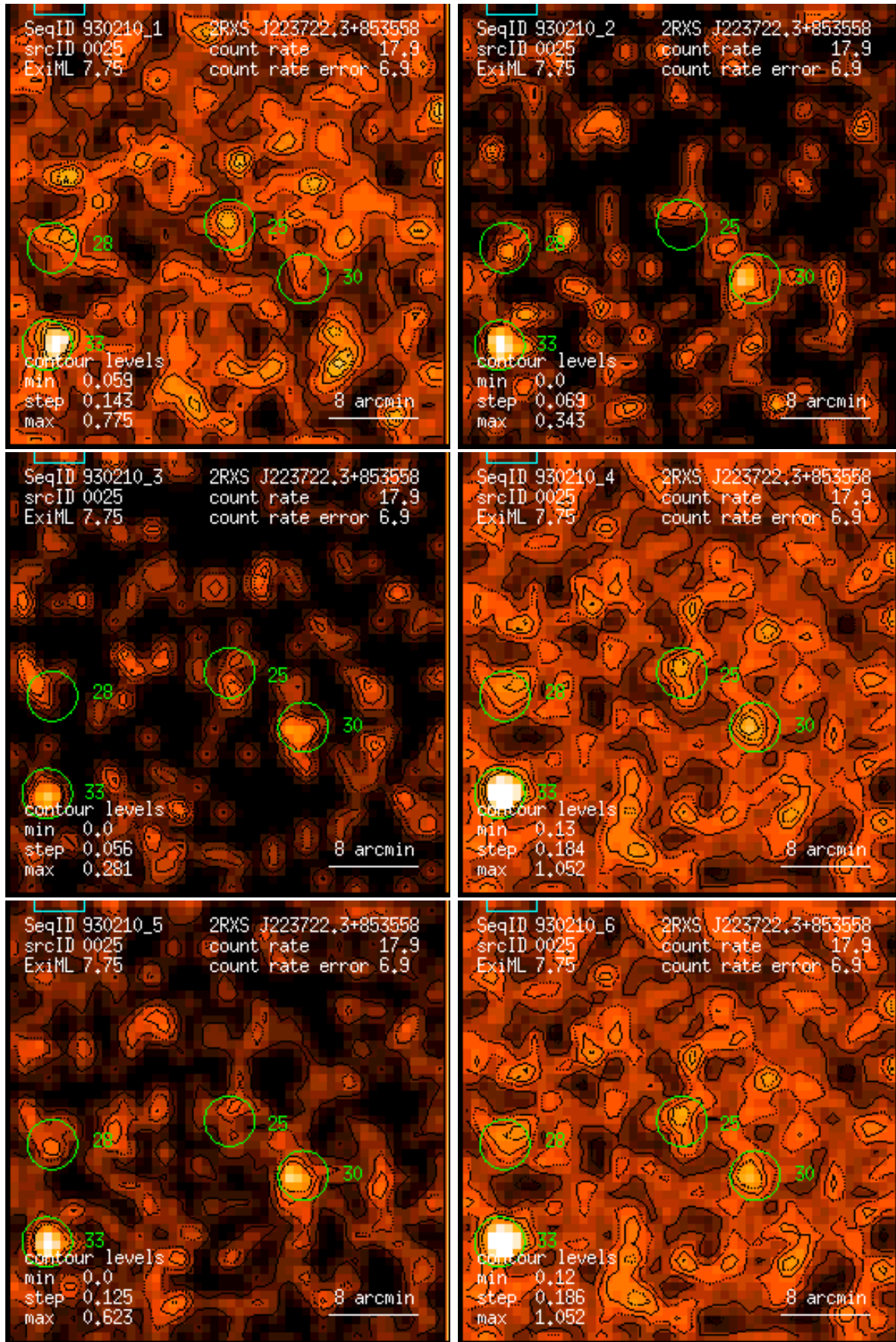
Figure 25: RASS 930210: detection 0025: band rate images, Gaussian filter: (1) PSPC channels 11 – 41, (2) 52 – 90, (3) 91 – 201, (4) 11 – 235, (5) 52 – 201, (6) 11 – 201. Broad band rates in counts/ks. Band rate contour levels in counts/ks/arcmin 2 .
