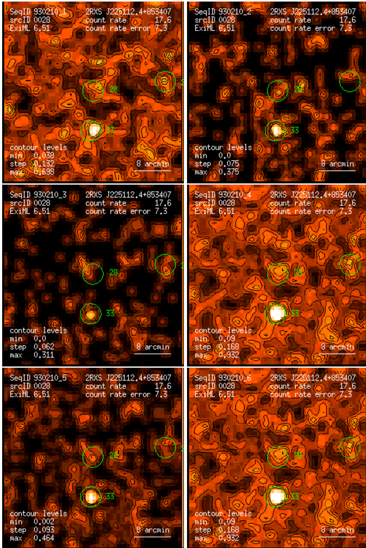
Figure 28: RASS 930210: detection 0028: band rate images, Gaussian filter: (1) PSPC channels 11 – 41, (2) 52 – 90, (3) 91 – 201, (4) 11 – 235, (5) 52 – 201, (6) 11 – 201. Broad band rates in counts/ks. Band rate contour levels in counts/ks/arcmin 2 .
