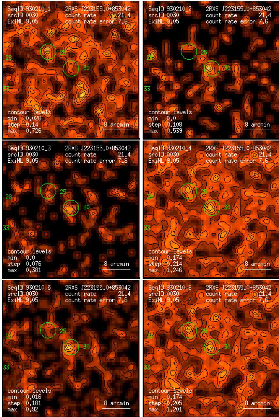
Figure 30: RASS 930210: detection 0030: band rate images, Gaussian filter: (1) PSPC channels 11 – 41, (2) 52 – 90, (3) 91 – 201, (4) 11 – 235, (5) 52 – 201, (6) 11 – 201. Broad band rates in counts/ks. Band rate contour levels in counts/ks/arcmin 2 .
