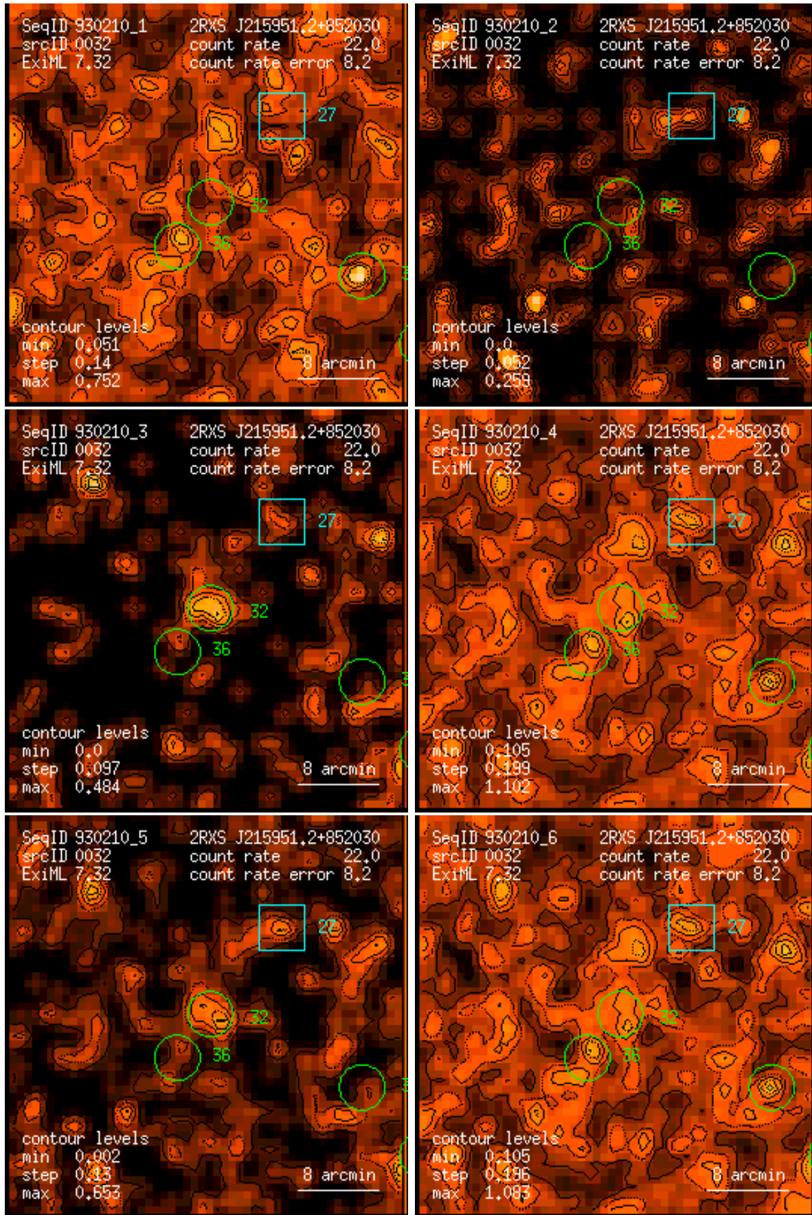
Figure 32: RASS 930210: detection 0032: band rate images, Gaussian filter: (1) PSPC channels 11 – 41, (2) 52 – 90, (3) 91 – 201, (4) 11 – 235, (5) 52 – 201, (6) 11 – 201. Broad band rates in counts/ks. Band rate contour levels in counts/ks/arcmin 2 .
