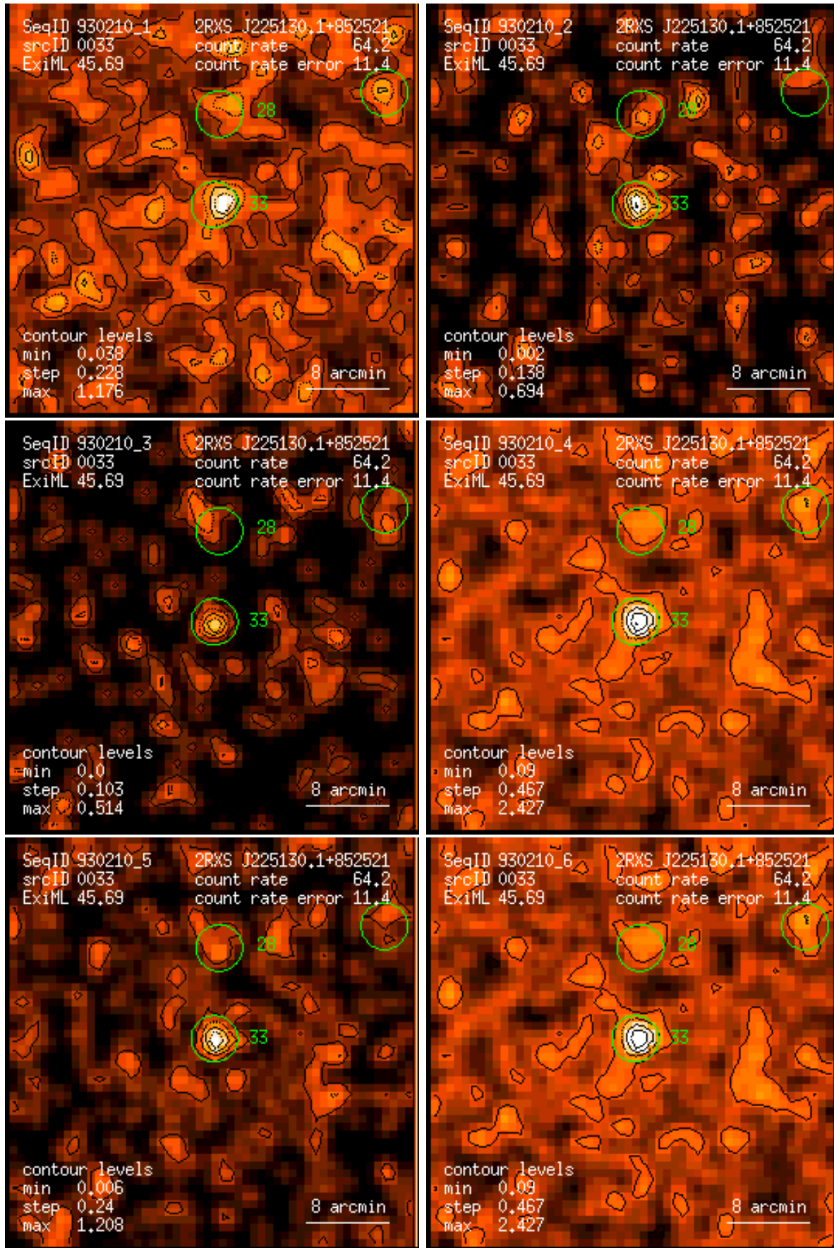
Figure 33: RASS 930210: detection 0033: band rate images, Gaussian filter: (1) PSPC channels 11 – 41, (2) 52 – 90, (3) 91 – 201, (4) 11 – 235, (5) 52 – 201, (6) 11 – 201. Broad band rates in counts/ks. Band rate contour levels in counts/ks/arcmin 2 .
