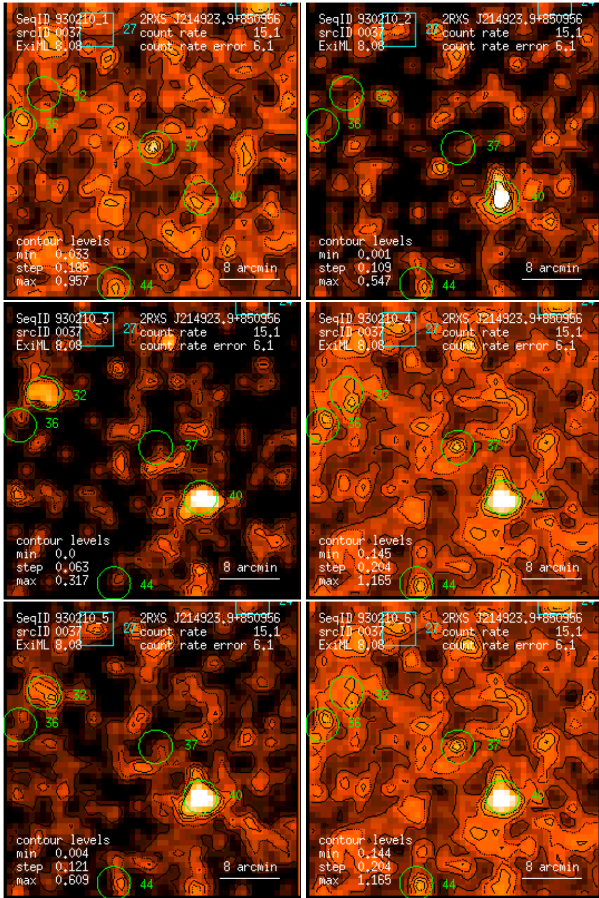
Figure 37: RASS 930210: detection 0037: band rate images, Gaussian filter: (1) PSPC channels 11 – 41, (2) 52 – 90, (3) 91 – 201, (4) 11 – 235, (5) 52 – 201, (6) 11 – 201. Broad band rates in counts/ks. Band rate contour levels in counts/ks/arcmin 2 .
