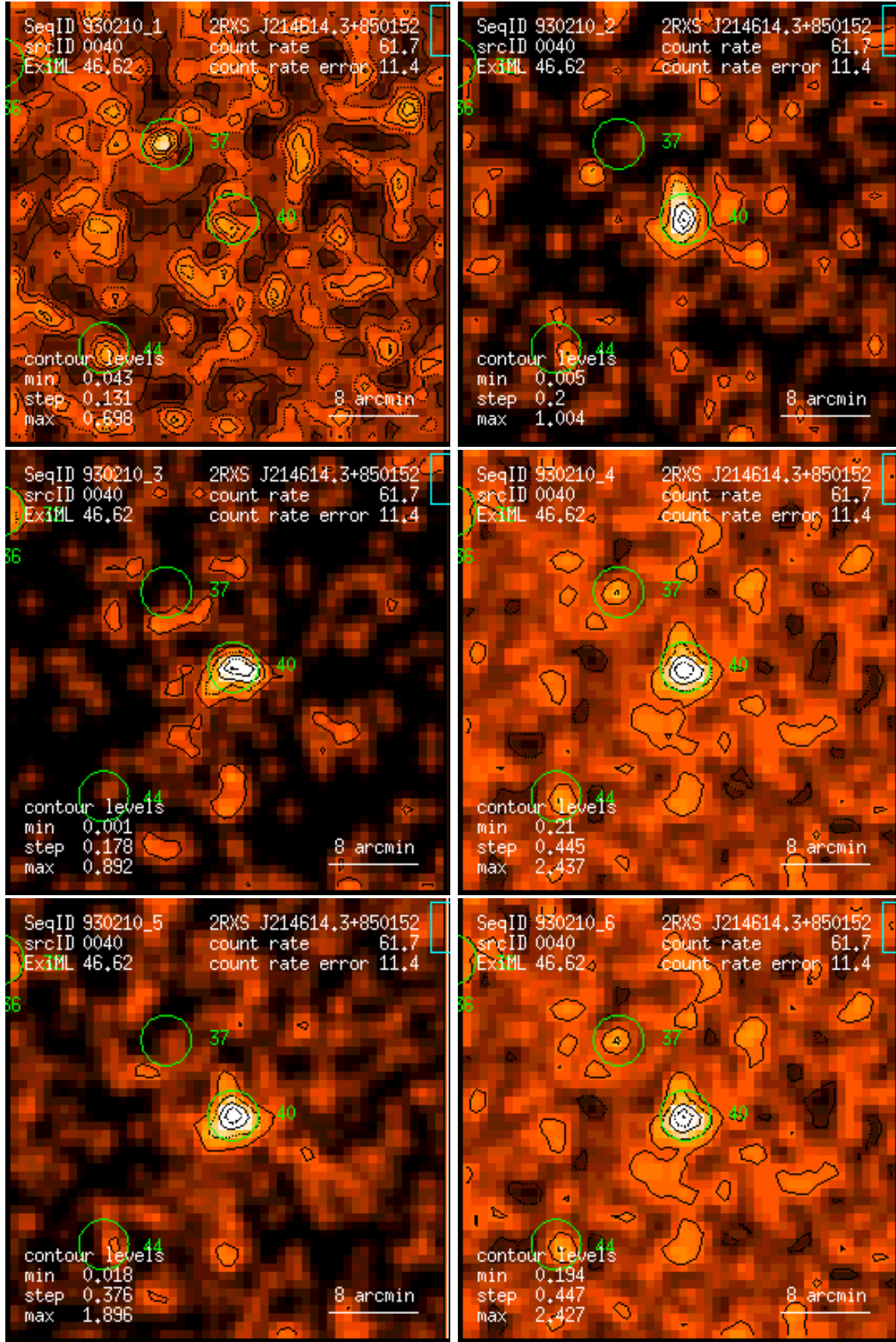
Figure 40: RASS 930210: detection 0040: band rate images, Gaussian filter: (1) PSPC channels 11 – 41, (2) 52 – 90, (3) 91 – 201, (4) 11 – 235, (5) 52 – 201, (6) 11 – 201. Broad band rates in counts/ks. Band rate contour levels in counts/ks/arcmin 2 .
