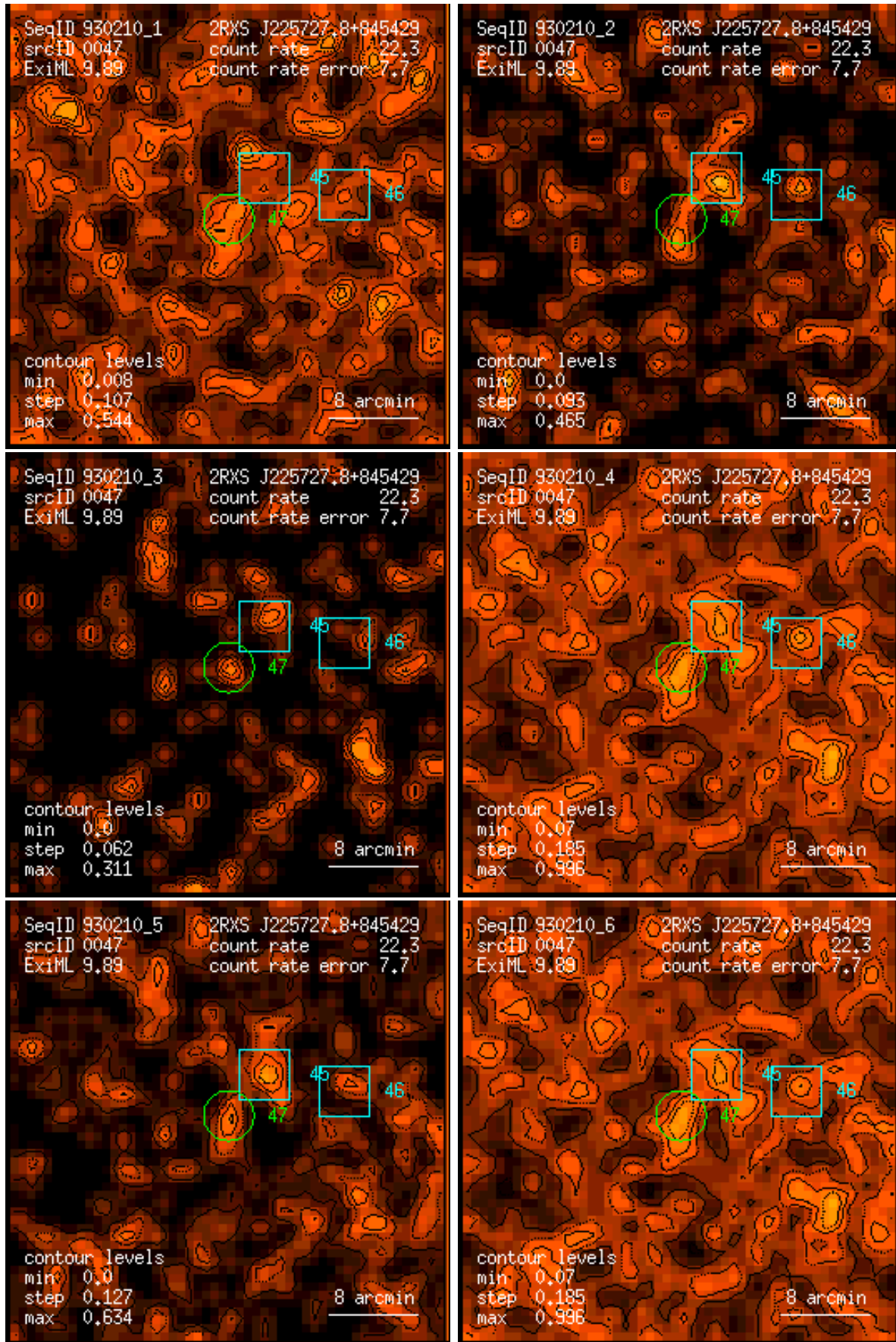
Figure 47: RASS 930210: detection 0047: band rate images, Gaussian filter: (1) PSPC channels 11 – 41, (2) 52 – 90, (3) 91 – 201, (4) 11 – 235, (5) 52 – 201, (6) 11 – 201. Broad band rates in counts/ks. Band rate contour levels in counts/ks/arcmin 2 .
