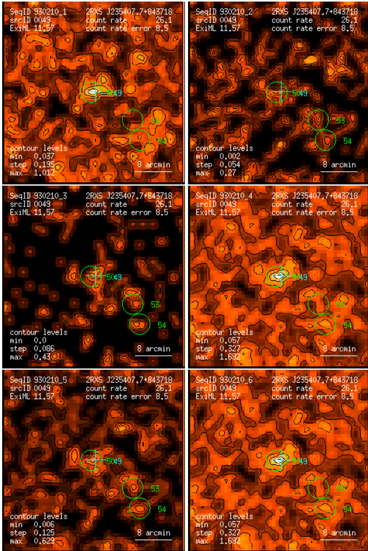
Figure 49: RASS 930210: detection 0049: band rate images, Gaussian filter: (1) PSPC channels 11 – 41, (2) 52 – 90, (3) 91 – 201, (4) 11 – 235, (5) 52 – 201, (6) 11 – 201. Broad band rates in counts/ks. Band rate contour levels in counts/ks/arcmin 2 .
