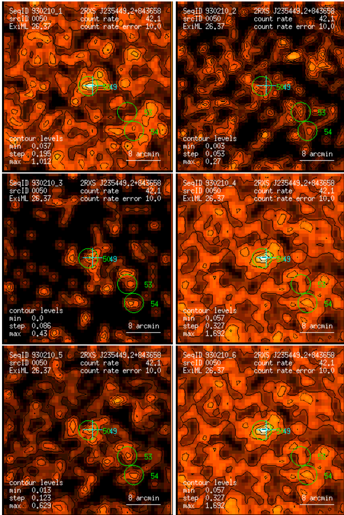
Figure 50: RASS 930210: detection 0050: band rate images, Gaussian filter: (1) PSPC channels 11 – 41, (2) 52 – 90, (3) 91 – 201, (4) 11 – 235, (5) 52 – 201, (6) 11 – 201. Broad band rates in counts/ks. Band rate contour levels in counts/ks/arcmin 2 .
