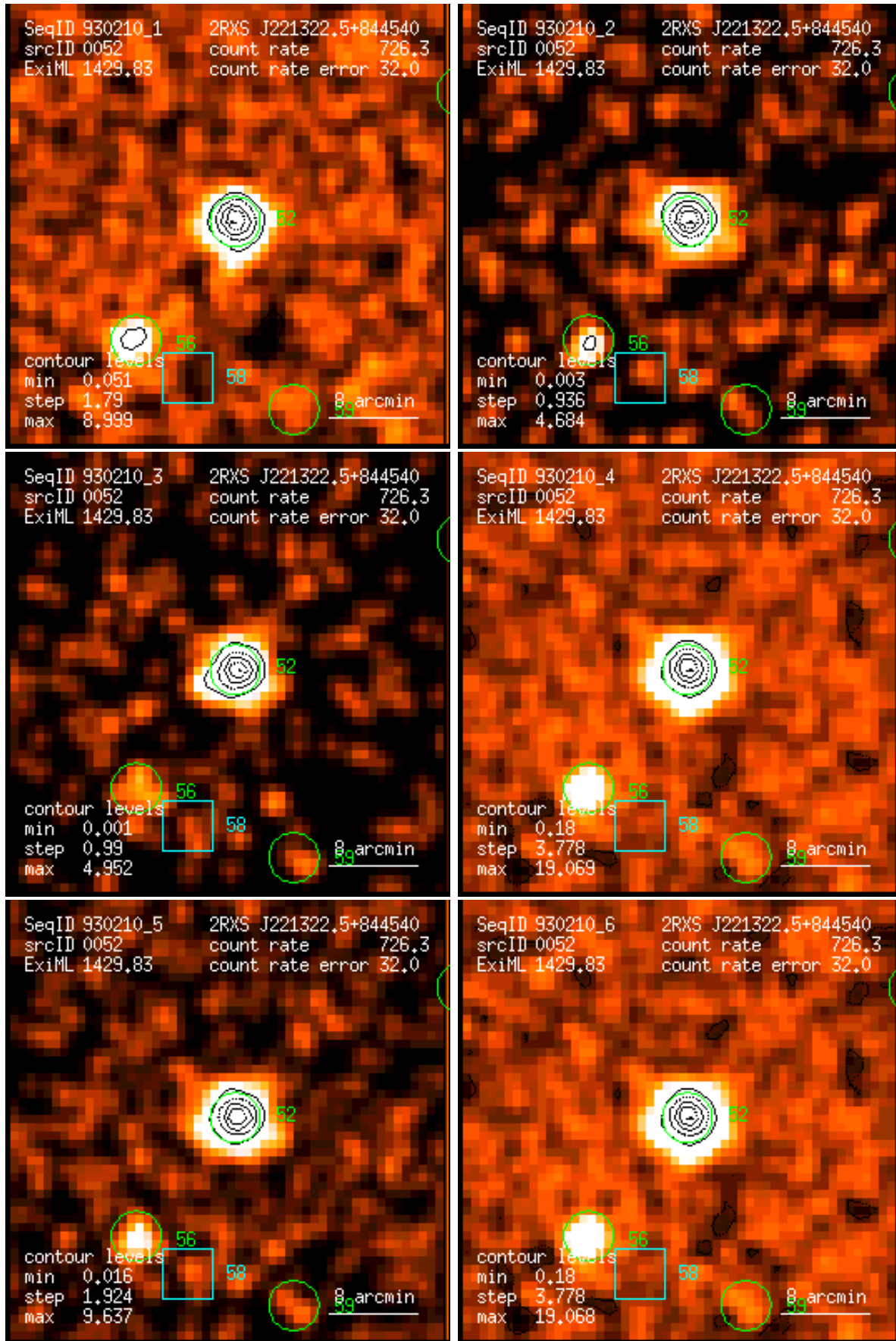
Figure 52: RASS 930210: detection 0052: band rate images, Gaussian filter: (1) PSPC channels 11 – 41, (2) 52 – 90, (3) 91 – 201, (4) 11 – 235, (5) 52 – 201, (6) 11 – 201. Broad band rates in counts/ks. Band rate contour levels in counts/ks/arcmin 2 .
