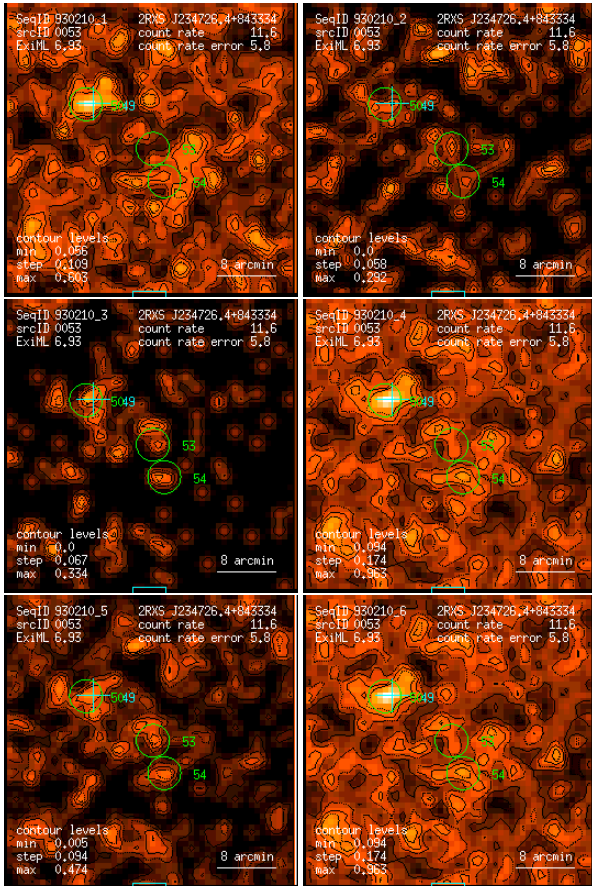
Figure 53: RASS 930210: detection 0053: band rate images, Gaussian filter: (1) PSPC channels 11 – 41, (2) 52 – 90, (3) 91 – 201, (4) 11 – 235, (5) 52 – 201, (6) 11 – 201. Broad band rates in counts/ks. Band rate contour levels in counts/ks/arcmin 2 .
