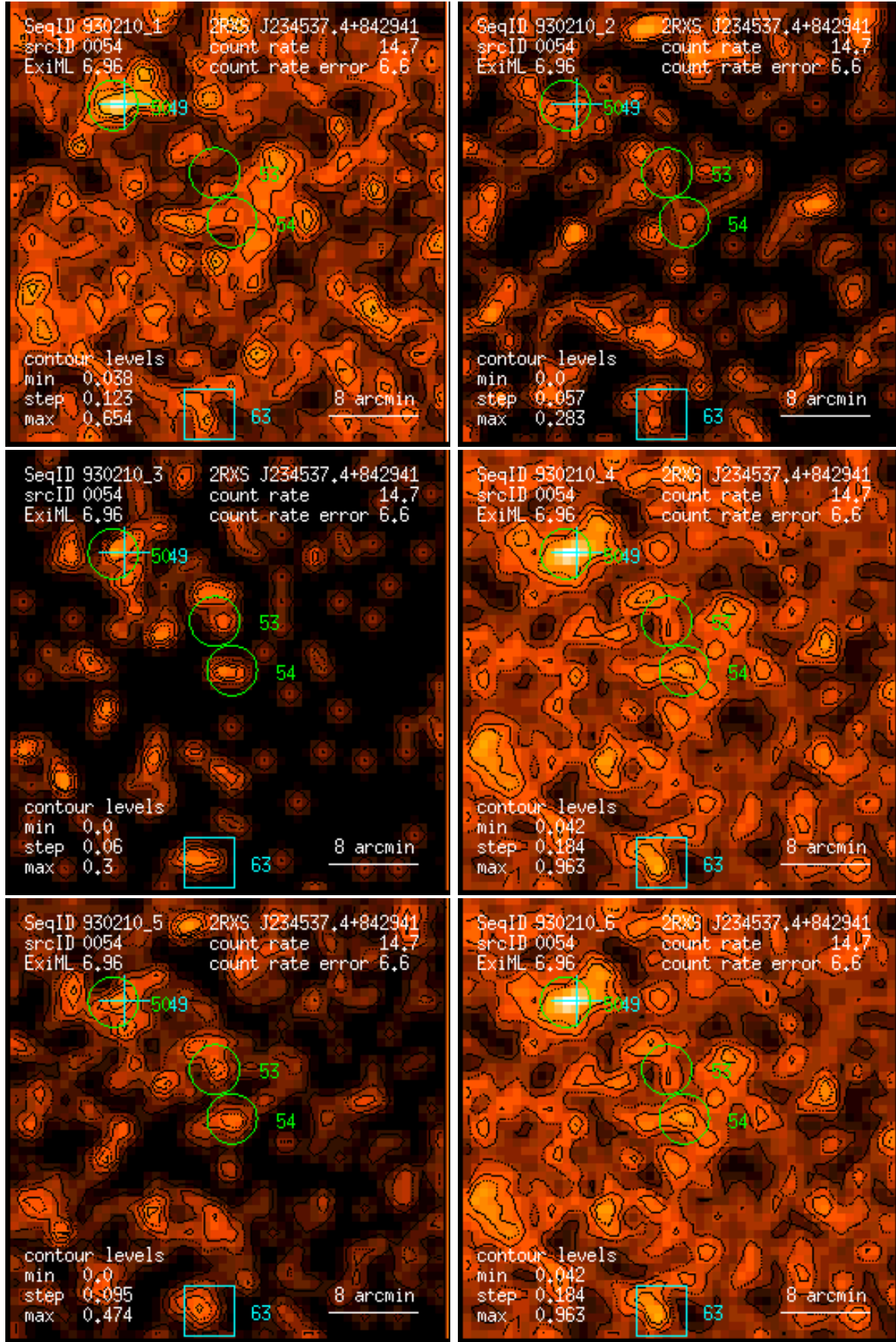
Figure 54: RASS 930210: detection 0054: band rate images, Gaussian filter: (1) PSPC channels 11 – 41, (2) 52 – 90, (3) 91 – 201, (4) 11 – 235, (5) 52 – 201, (6) 11 – 201. Broad band rates in counts/ks. Band rate contour levels in counts/ks/arcmin 2 .
