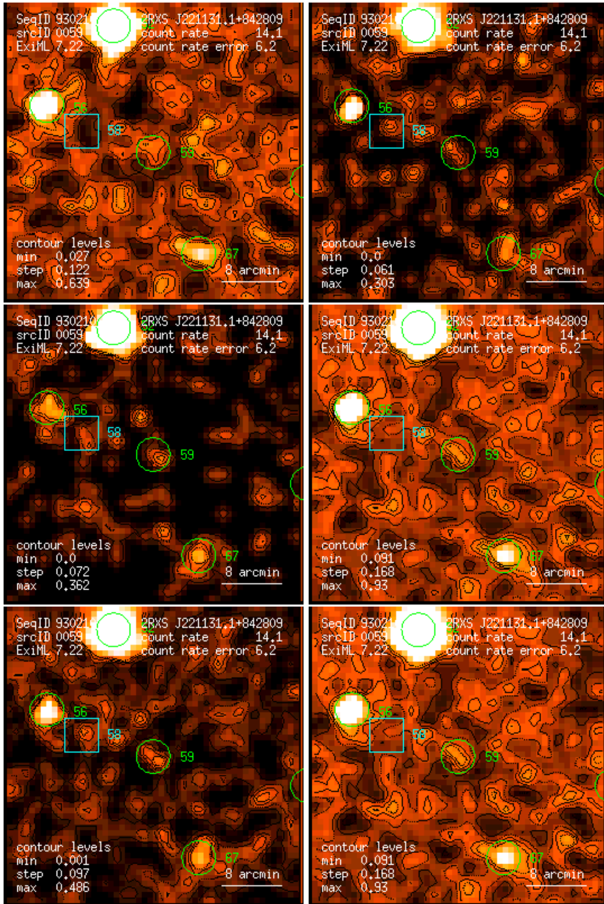
Figure 59: RASS 930210: detection 0059: band rate images, Gaussian filter: (1) PSPC channels 11 – 41, (2) 52 – 90, (3) 91 – 201, (4) 11 – 235, (5) 52 – 201, (6) 11 – 201. Broad band rates in counts/ks. Band rate contour levels in counts/ks/arcmin 2 .
