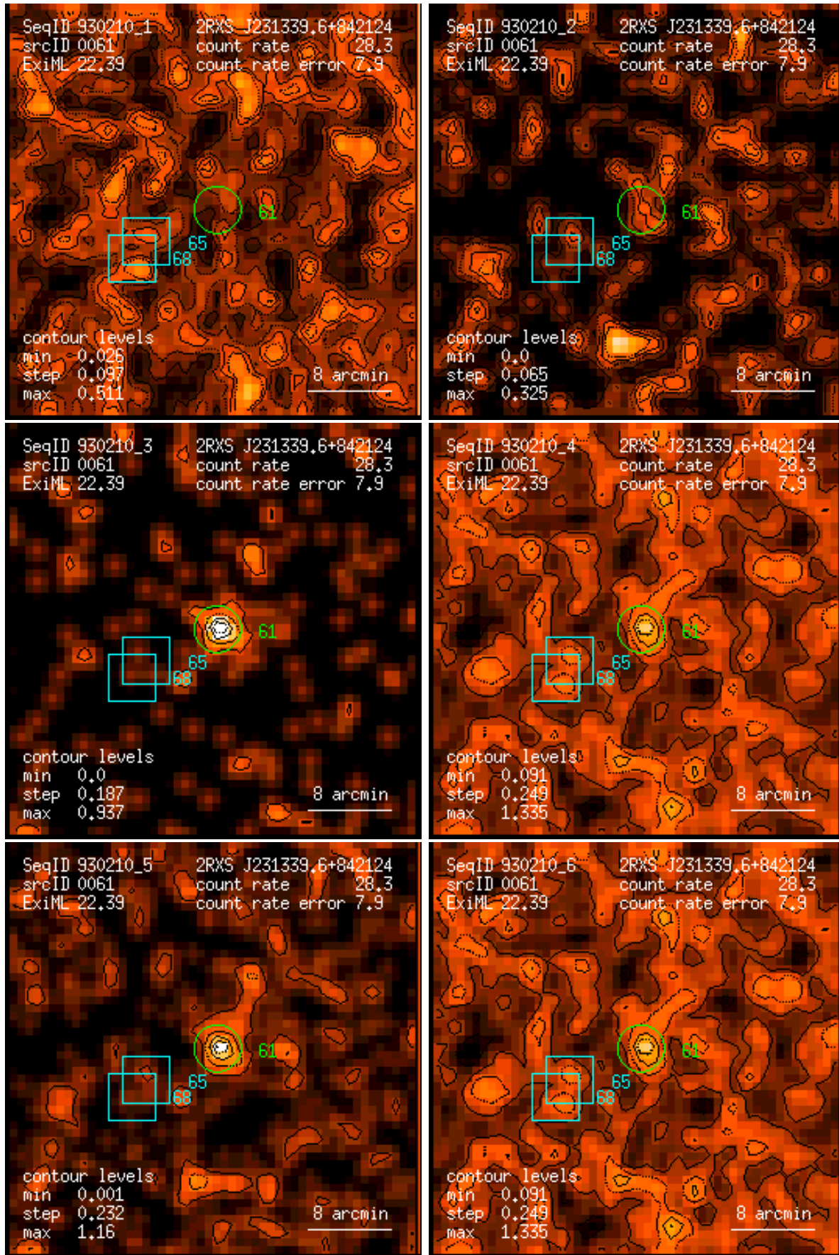
Figure 61: RASS 930210: detection 0061: band rate images, Gaussian filter: (1) PSPC channels 11 – 41, (2) 52 – 90, (3) 91 – 201, (4) 11 – 235, (5) 52 – 201, (6) 11 – 201. Broad band rates in counts/ks. Band rate contour levels in counts/ks/arcmin 2 .
