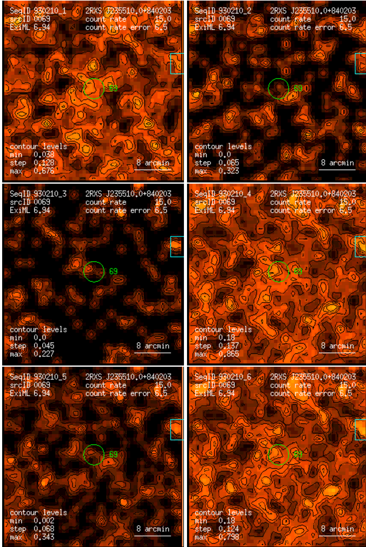
Figure 69: RASS 930210: detection 0069: band rate images, Gaussian filter: (1) PSPC channels 11 – 41, (2) 52 – 90, (3) 91 – 201, (4) 11 – 235, (5) 52 – 201, (6) 11 – 201. Broad band rates in counts/ks. Band rate contour levels in counts/ks/arcmin 2 .
