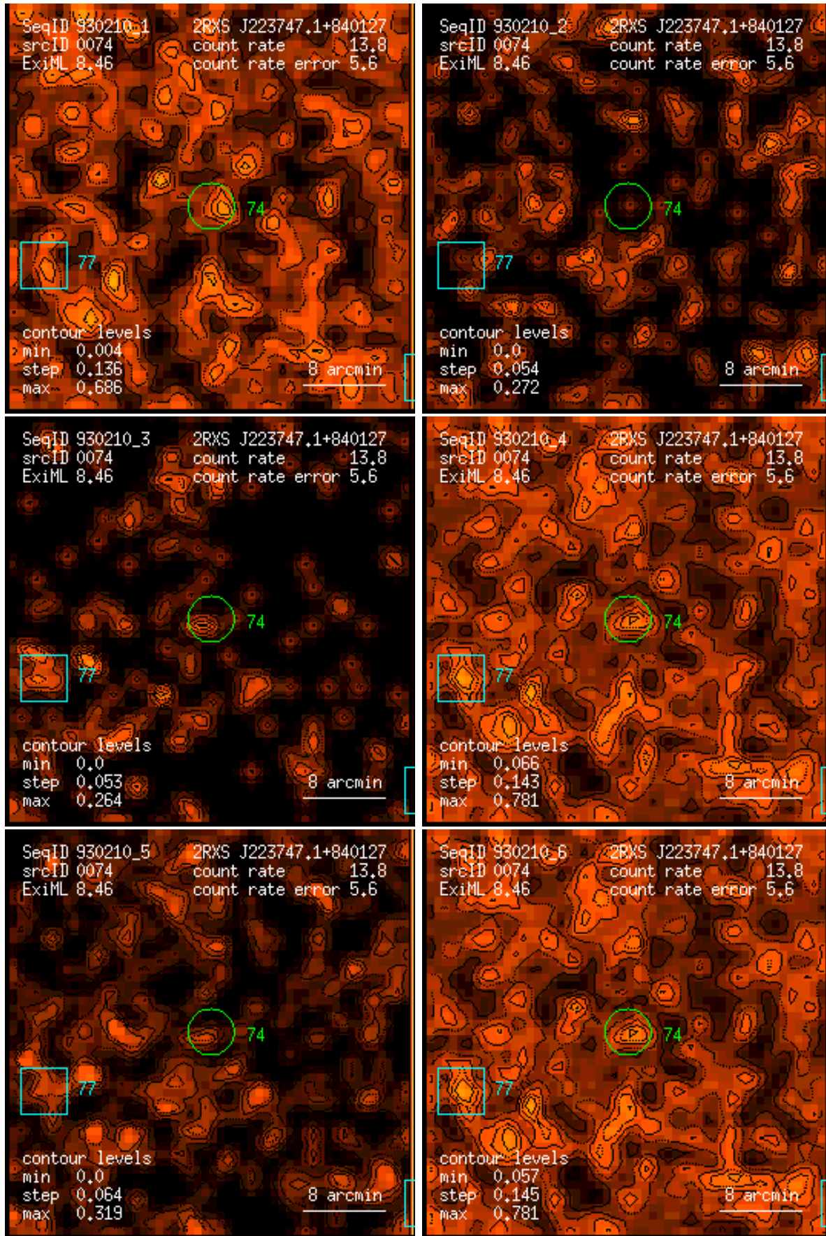
Figure 74: RASS 930210: detection 0074: band rate images, Gaussian filter: (1) PSPC channels 11 – 41, (2) 52 – 90, (3) 91 – 201, (4) 11 – 235, (5) 52 – 201, (6) 11 – 201. Broad band rates in counts/ks. Band rate contour levels in counts/ks/arcmin 2 .
