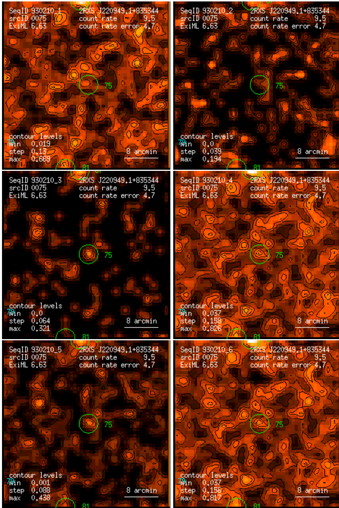
Figure 75: RASS 930210: detection 0075: band rate images, Gaussian filter: (1) PSPC channels 11 – 41, (2) 52 – 90, (3) 91 – 201, (4) 11 – 235, (5) 52 – 201, (6) 11 – 201. Broad band rates in counts/ks. Band rate contour levels in counts/ks/arcmin 2 .
