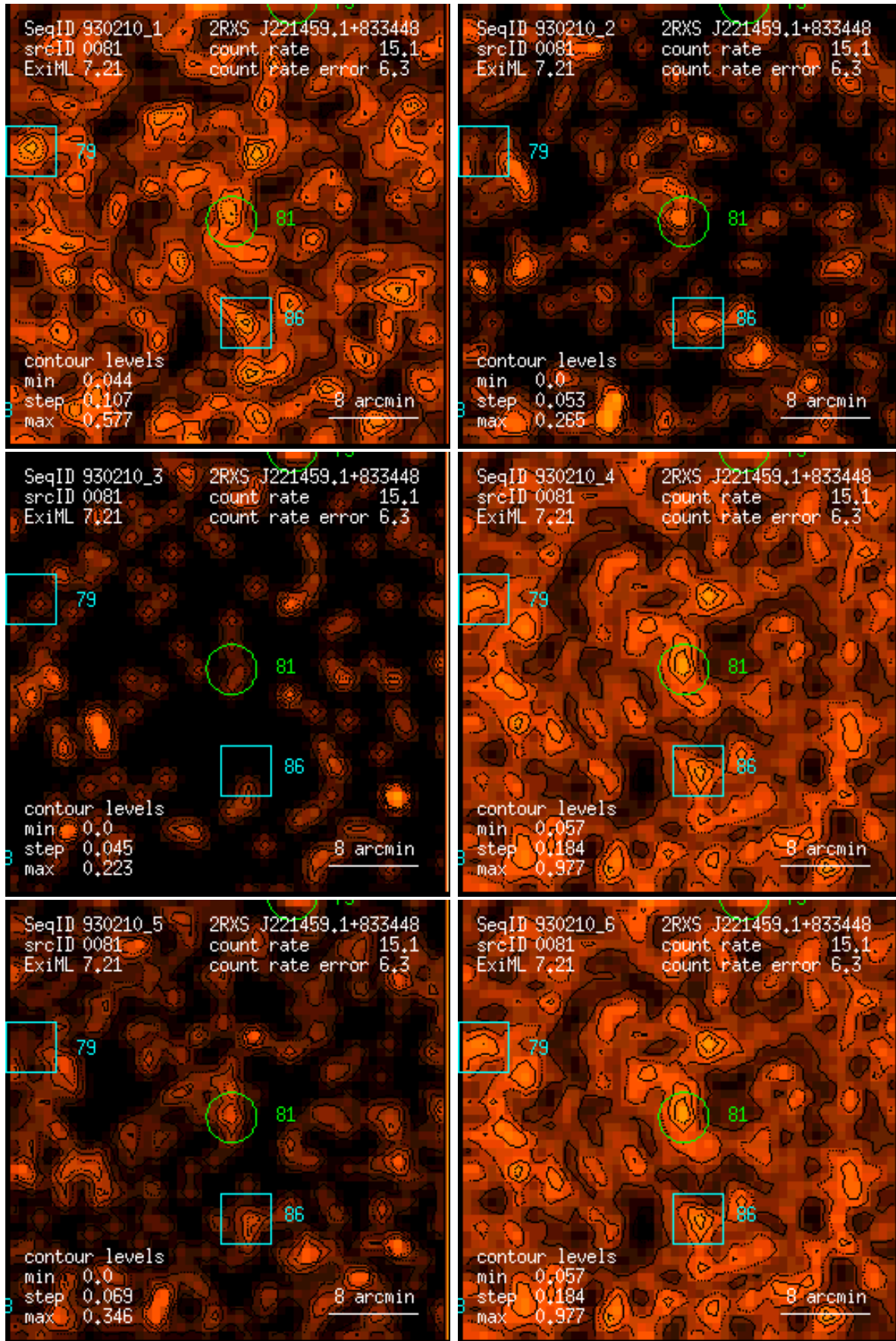
Figure 81: RASS 930210: detection 0081: band rate images, Gaussian filter: (1) PSPC channels 11 – 41, (2) 52 – 90, (3) 91 – 201, (4) 11 – 235, (5) 52 – 201, (6) 11 – 201. Broad band rates in counts/ks. Band rate contour levels in counts/ks/arcmin 2 .
