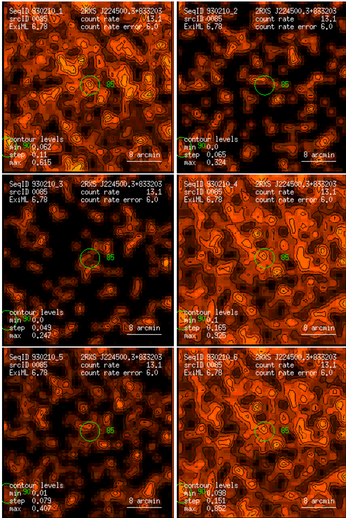
Figure 85: RASS 930210: detection 0085: band rate images, Gaussian filter: (1) PSPC channels 11 – 41, (2) 52 – 90, (3) 91 – 201, (4) 11 – 235, (5) 52 – 201, (6) 11 – 201. Broad band rates in counts/ks. Band rate contour levels in counts/ks/arcmin 2 .
