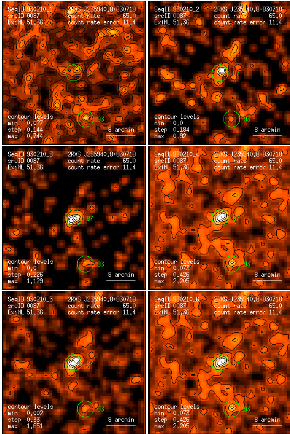
Figure 87: RASS 930210: detection 0087: band rate images, Gaussian filter: (1) PSPC channels 11 – 41, (2) 52 – 90, (3) 91 – 201, (4) 11 – 235, (5) 52 – 201, (6) 11 – 201. Broad band rates in counts/ks. Band rate contour levels in counts/ks/arcmin 2 .
