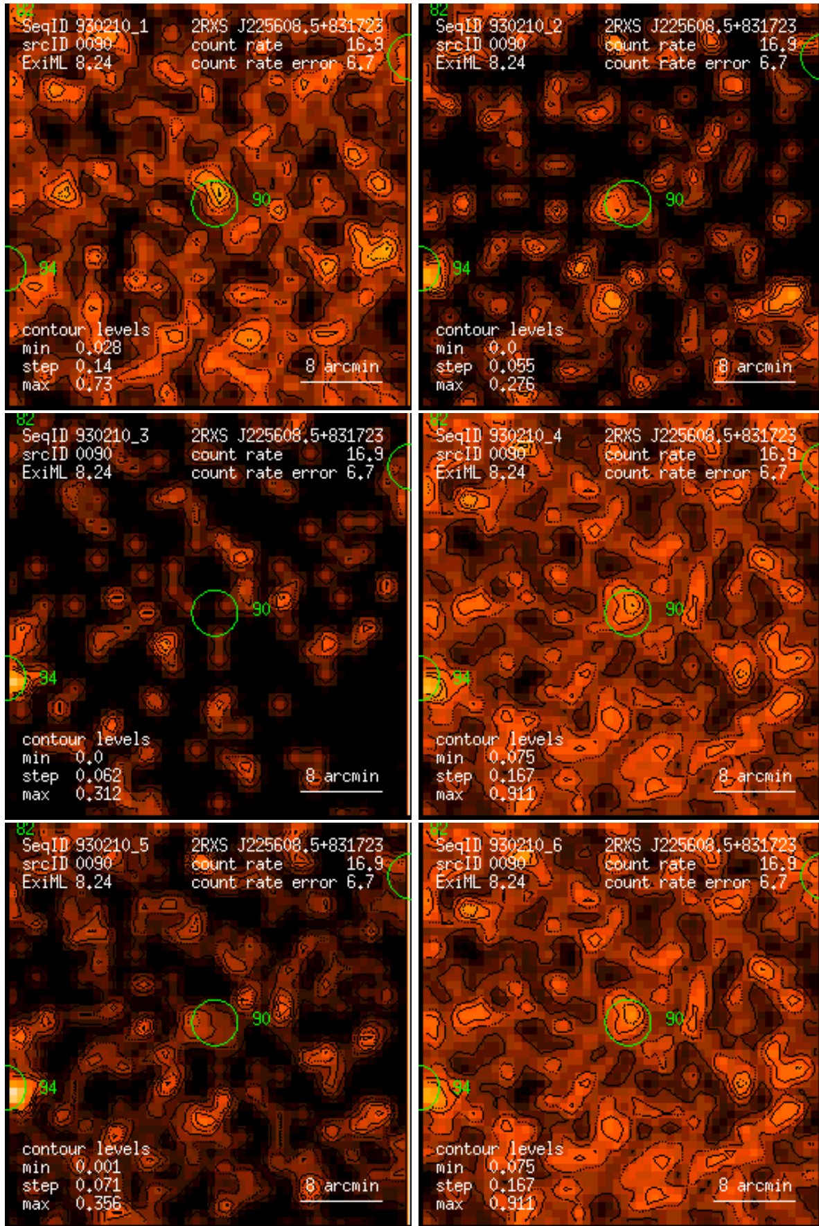
Figure 90: RASS 930210: detection 0090: band rate images, Gaussian filter: (1) PSPC channels 11 – 41, (2) 52 – 90, (3) 91 – 201, (4) 11 – 235, (5) 52 – 201, (6) 11 – 201. Broad band rates in counts/ks. Band rate contour levels in counts/ks/arcmin 2 .
