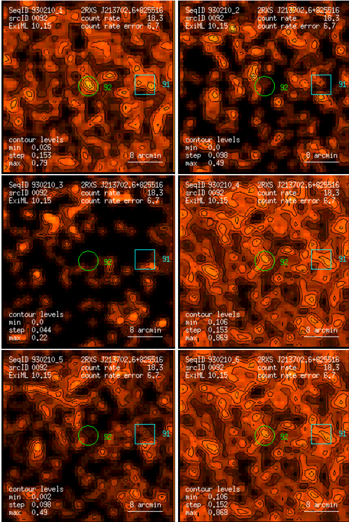
Figure 92: RASS 930210: detection 0092: band rate images, Gaussian filter: (1) PSPC channels 11 – 41, (2) 52 – 90, (3) 91 – 201, (4) 11 – 235, (5) 52 – 201, (6) 11 – 201. Broad band rates in counts/ks. Band rate contour levels in counts/ks/arcmin 2 .
