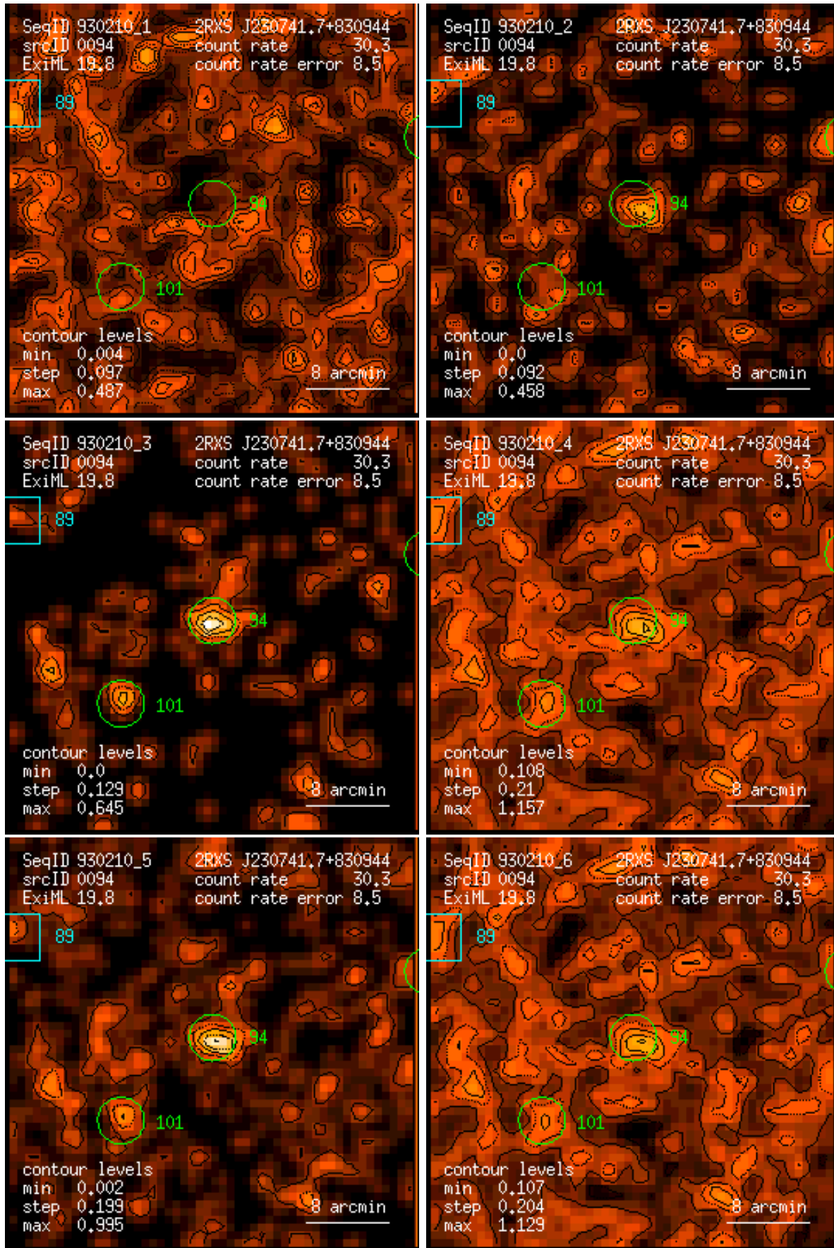
Figure 94: RASS 930210: detection 0094: band rate images, Gaussian filter: (1) PSPC channels 11 – 41, (2) 52 – 90, (3) 91 – 201, (4) 11 – 235, (5) 52 – 201, (6) 11 – 201. Broad band rates in counts/ks. Band rate contour levels in counts/ks/arcmin 2 .
