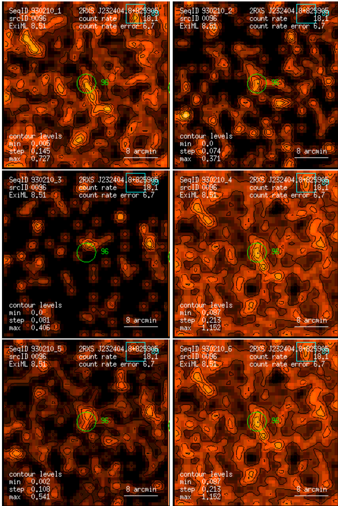
Figure 96: RASS 930210: detection 0096: band rate images, Gaussian filter: (1) PSPC channels 11 – 41, (2) 52 – 90, (3) 91 – 201, (4) 11 – 235, (5) 52 – 201, (6) 11 – 201. Broad band rates in counts/ks. Band rate contour levels in counts/ks/arcmin 2 .
