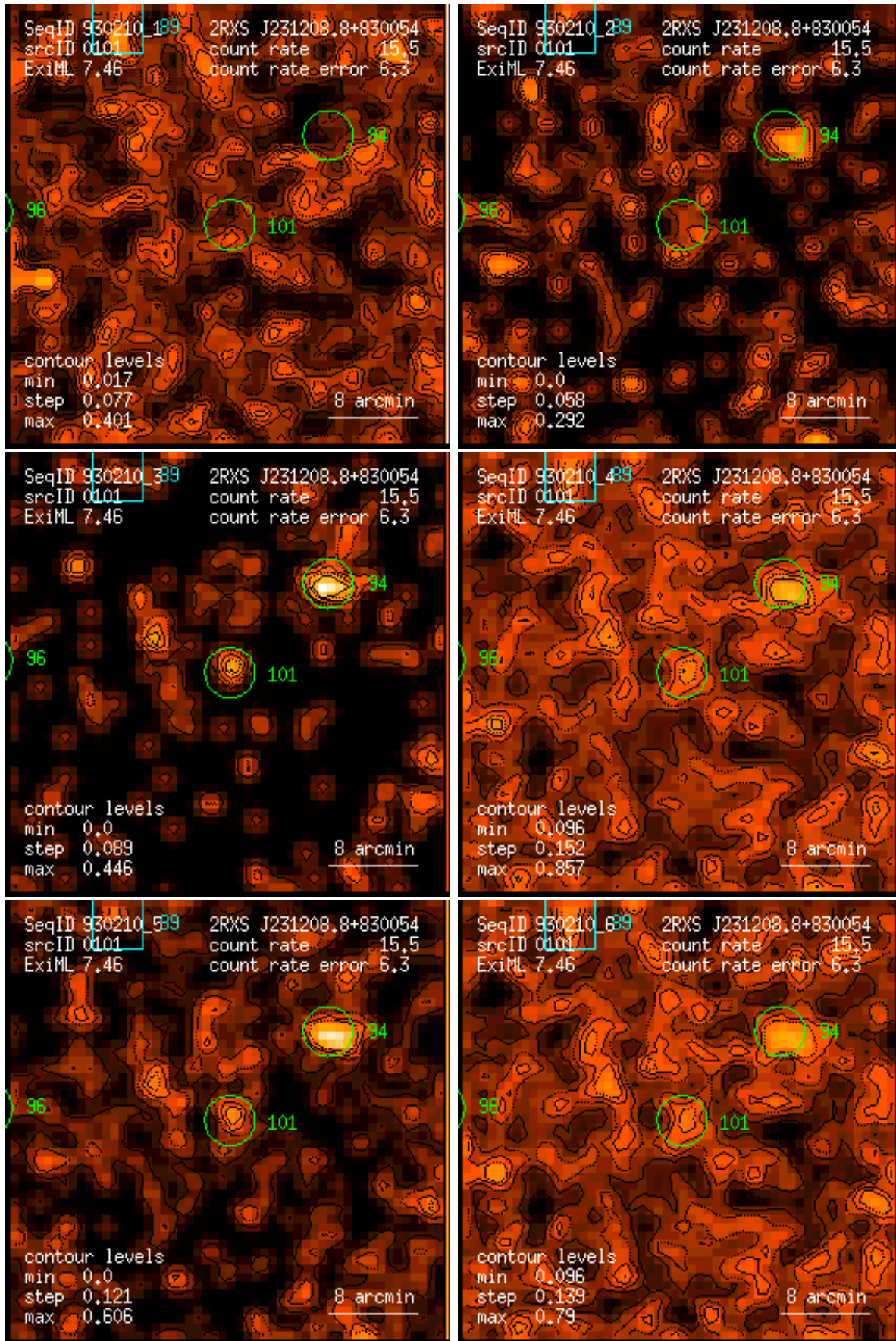
Figure 101: RASS 930210: detection 0101: band rate images, Gaussian filter: (1) PSPC channels 11 – 41, (2) 52 – 90, (3) 91 – 201, (4) 11 – 235, (5) 52 – 201, (6) 11 – 201. Broad band rates in counts/ks. Band rate contour levels in counts/ks/arcmin 2 .
