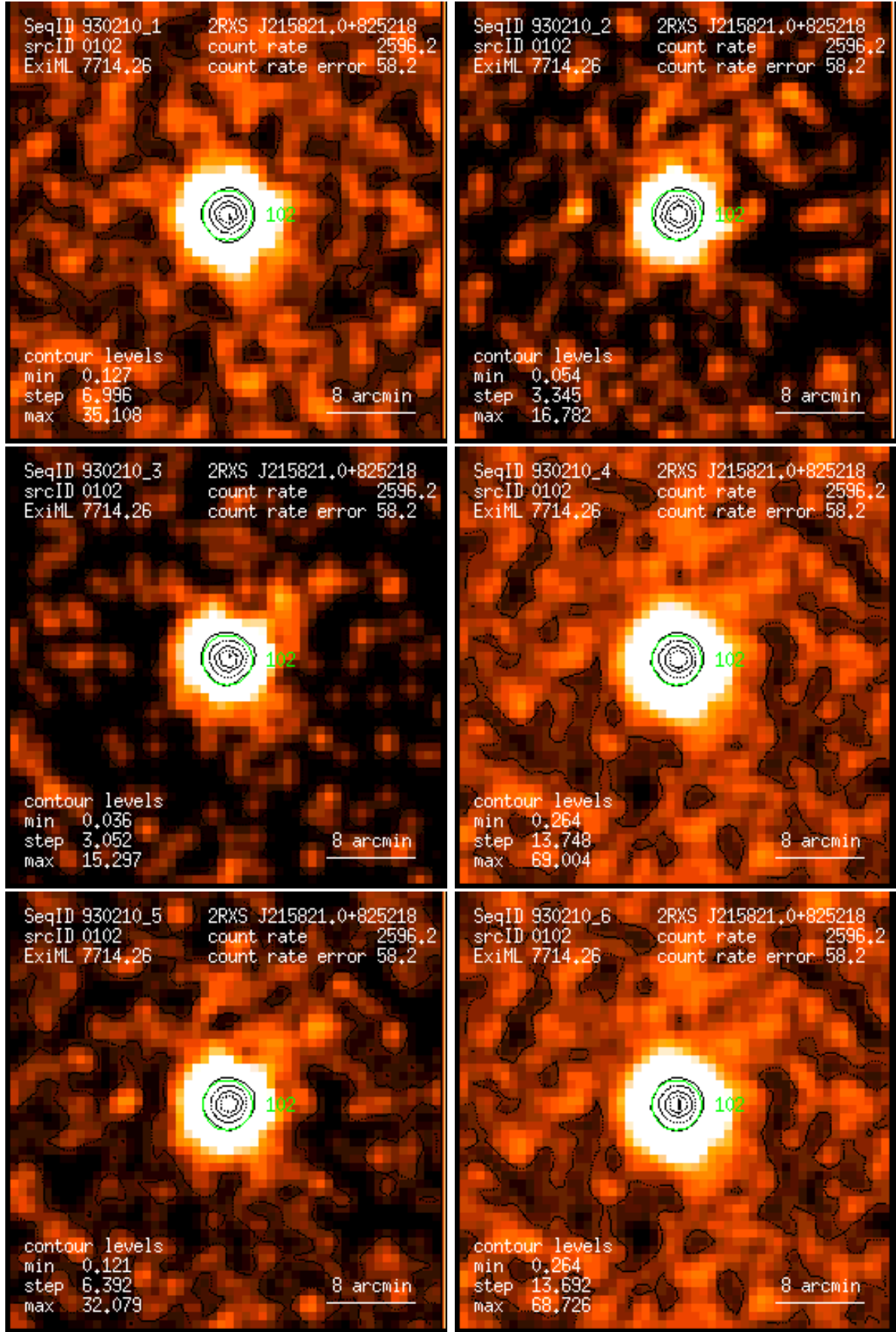
Figure 102: RASS 930210: detection 0102: band rate images, Gaussian filter: (1) PSPC channels 11 – 41, (2) 52 – 90, (3) 91 – 201, (4) 11 – 235, (5) 52 – 201, (6) 11 – 201. Broad band rates in counts/ks. Band rate contour levels in counts/ks/arcmin 2 .
