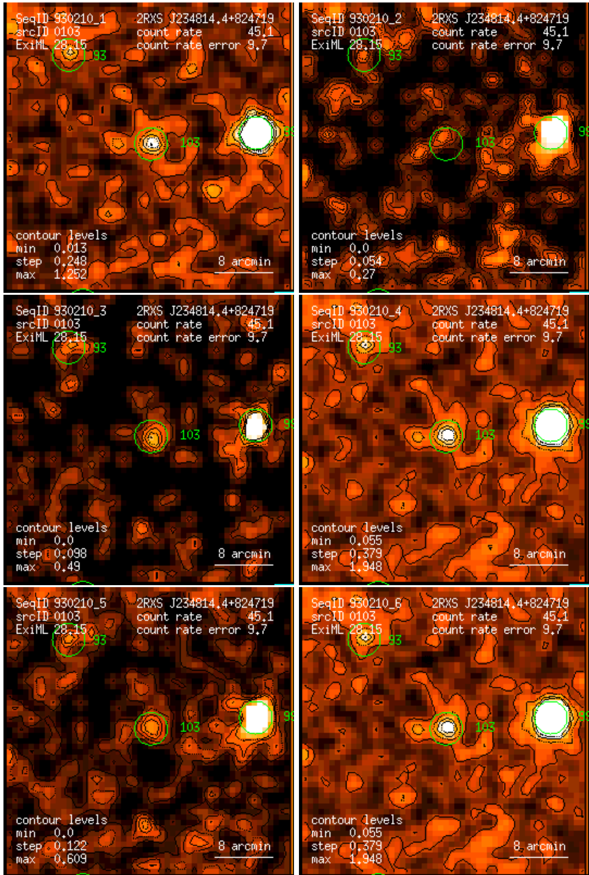
Figure 103: RASS 930210: detection 0103: band rate images, Gaussian filter: (1) PSPC channels 11 – 41, (2) 52 – 90, (3) 91 – 201, (4) 11 – 235, (5) 52 – 201, (6) 11 – 201. Broad band rates in counts/ks. Band rate contour levels in counts/ks/arcmin 2 .
