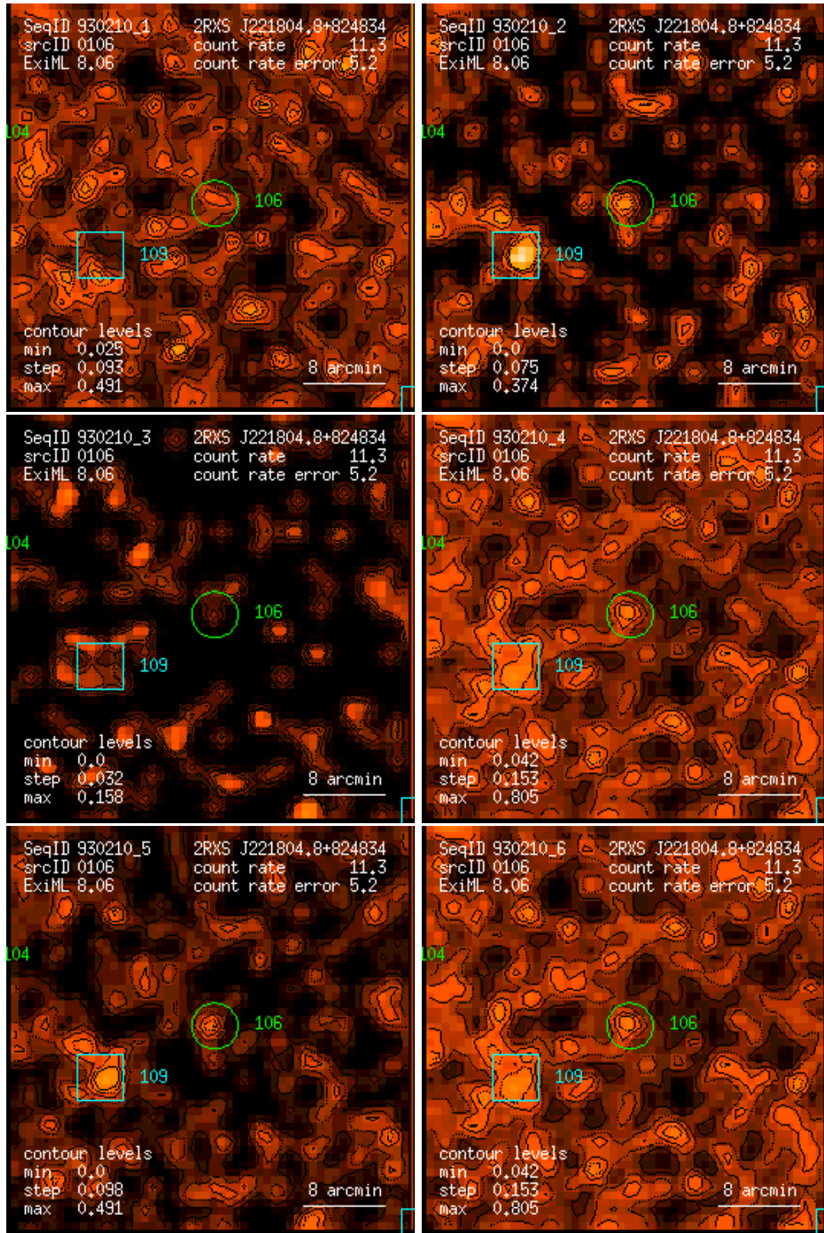
Figure 106: RASS 930210: detection 0106: band rate images, Gaussian filter: (1) PSPC channels 11 – 41, (2) 52 – 90, (3) 91 – 201, (4) 11 – 235, (5) 52 – 201, (6) 11 – 201. Broad band rates in counts/ks. Band rate contour levels in counts/ks/arcmin 2 .
