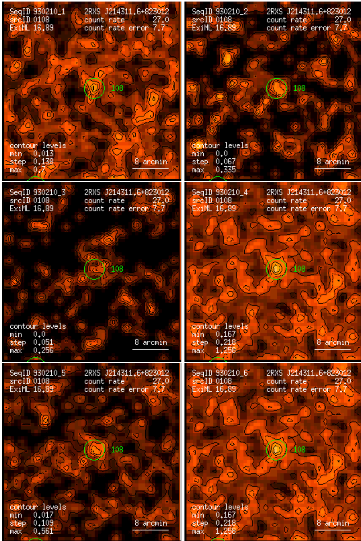
Figure 108: RASS 930210: detection 0108: band rate images, Gaussian filter: (1) PSPC channels 11 – 41, (2) 52 – 90, (3) 91 – 201, (4) 11 – 235, (5) 52 – 201, (6) 11 – 201. Broad band rates in counts/ks. Band rate contour levels in counts/ks/arcmin 2 .
