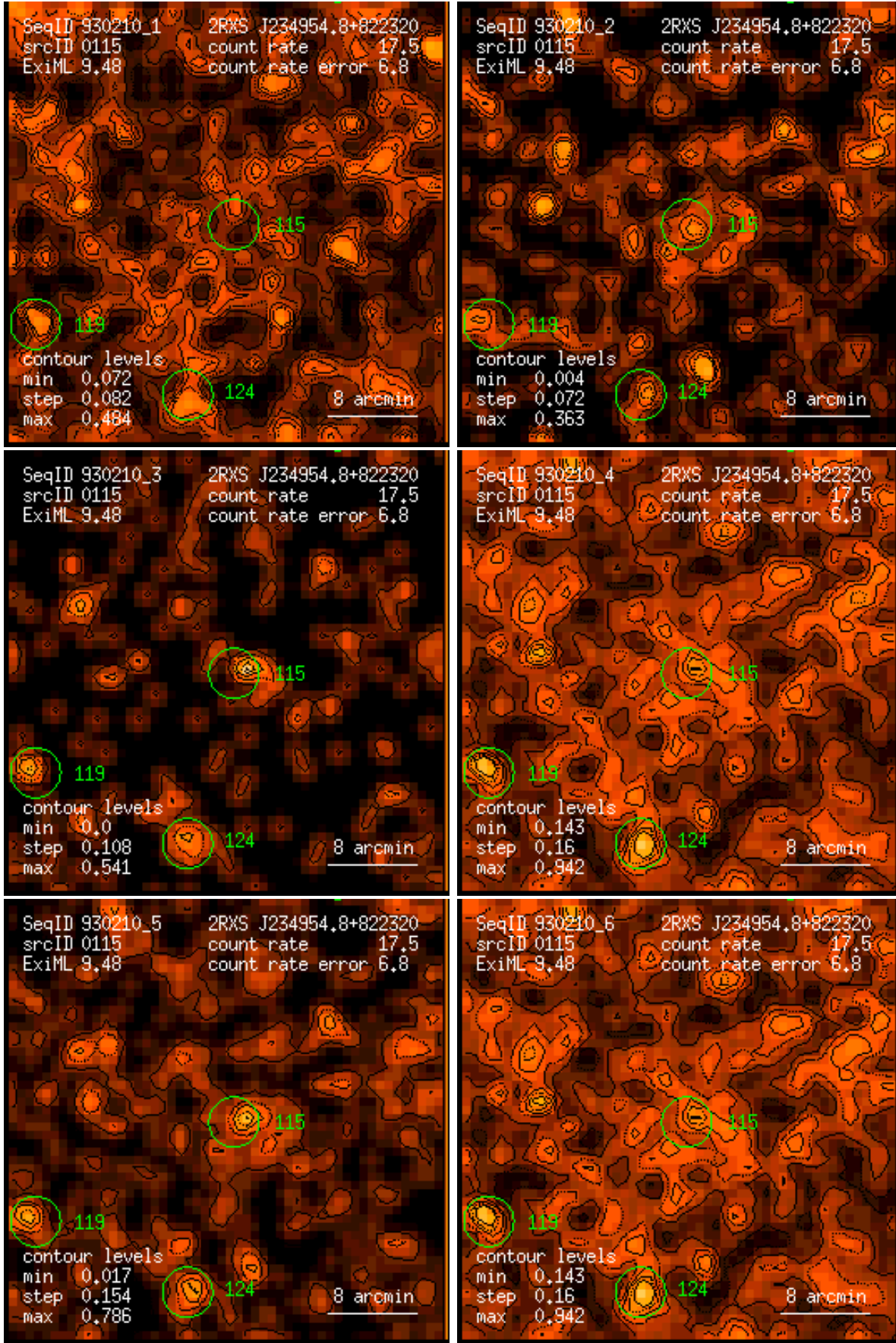
Figure 115: RASS 930210: detection 0115: band rate images, Gaussian filter: (1) PSPC channels 11 – 41, (2) 52 – 90, (3) 91 – 201, (4) 11 – 235, (5) 52 – 201, (6) 11 – 201. Broad band rates in counts/ks. Band rate contour levels in counts/ks/arcmin 2 .
