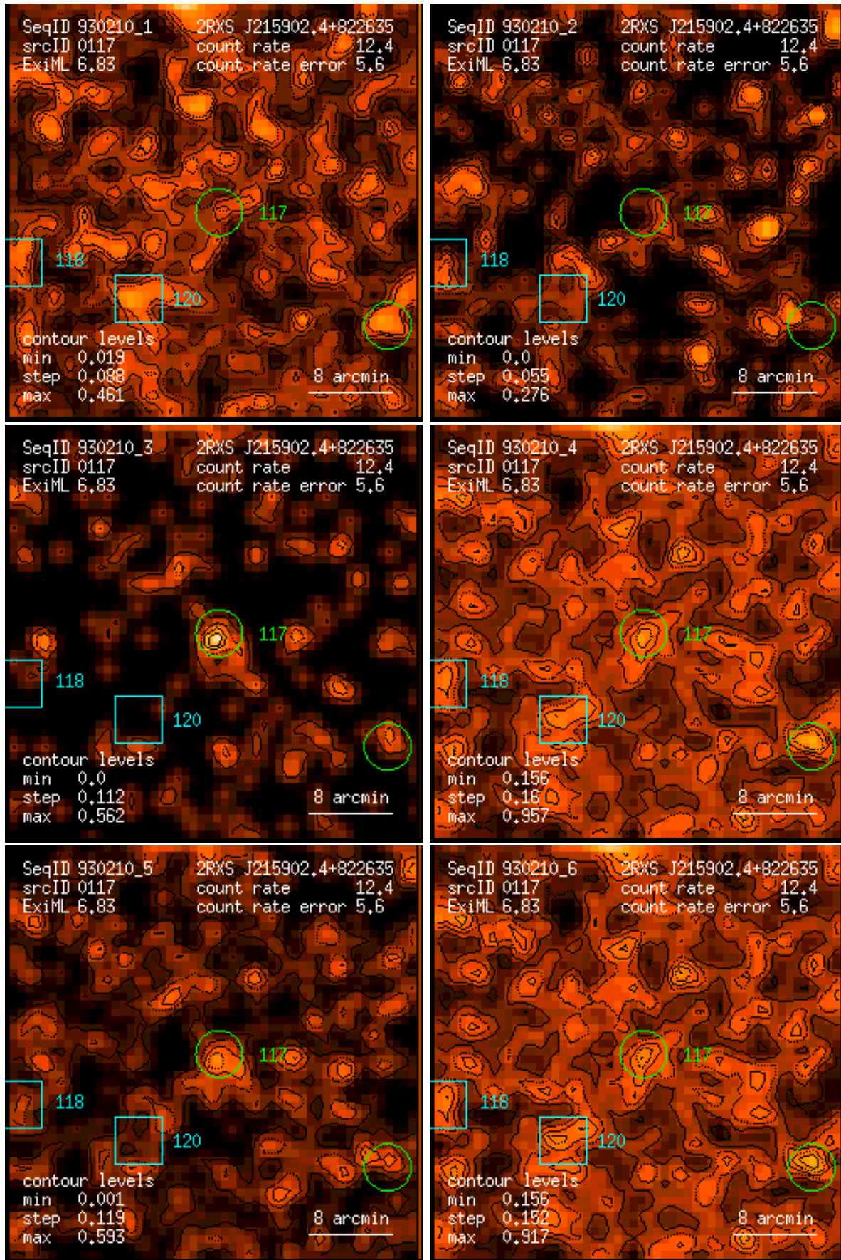
Figure 117: RASS 930210: detection 0117: band rate images, Gaussian filter: (1) PSPC channels 11 – 41, (2) 52 – 90, (3) 91 – 201, (4) 11 – 235, (5) 52 – 201, (6) 11 – 201. Broad band rates in counts/ks. Band rate contour levels in counts/ks/arcmin 2 .
