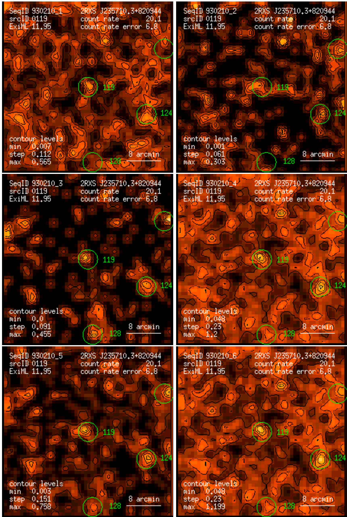
Figure 119: RASS 930210: detection 0119: band rate images, Gaussian filter: (1) PSPC channels 11 – 41, (2) 52 – 90, (3) 91 – 201, (4) 11 – 235, (5) 52 – 201, (6) 11 – 201. Broad band rates in counts/ks. Band rate contour levels in counts/ks/arcmin 2 .
